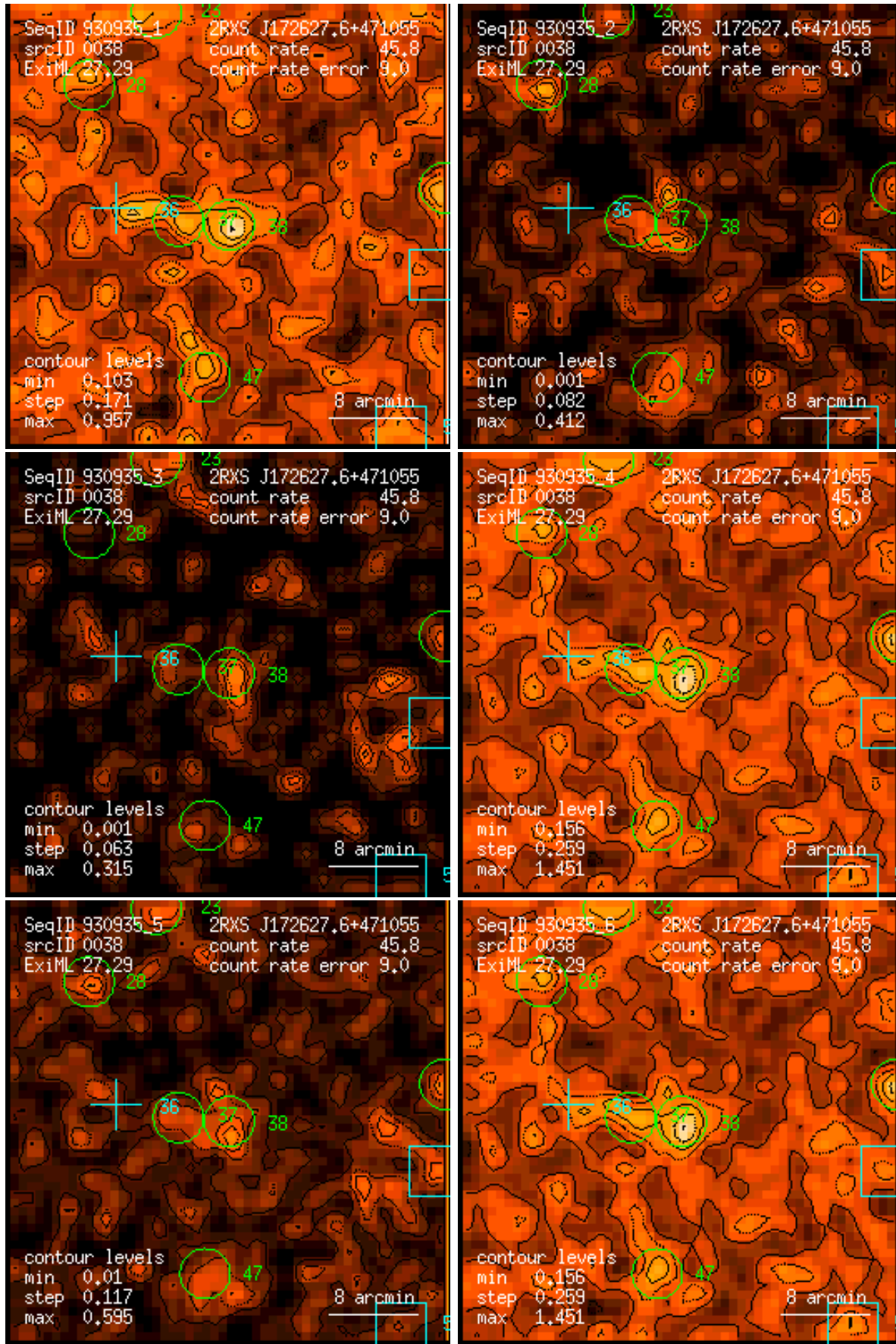
Figure 38: RASS 930935: detection 0038: band rate images, Gaussian filter: (1) PSPC channels 11 – 41, (2) 52 – 90, (3) 91 – 201, (4) 11 – 235, (5) 52 – 201, (6) 11 – 201. Broad band rates in counts/ks. Band rate contour levels in counts/ks/arcmin 2 .
