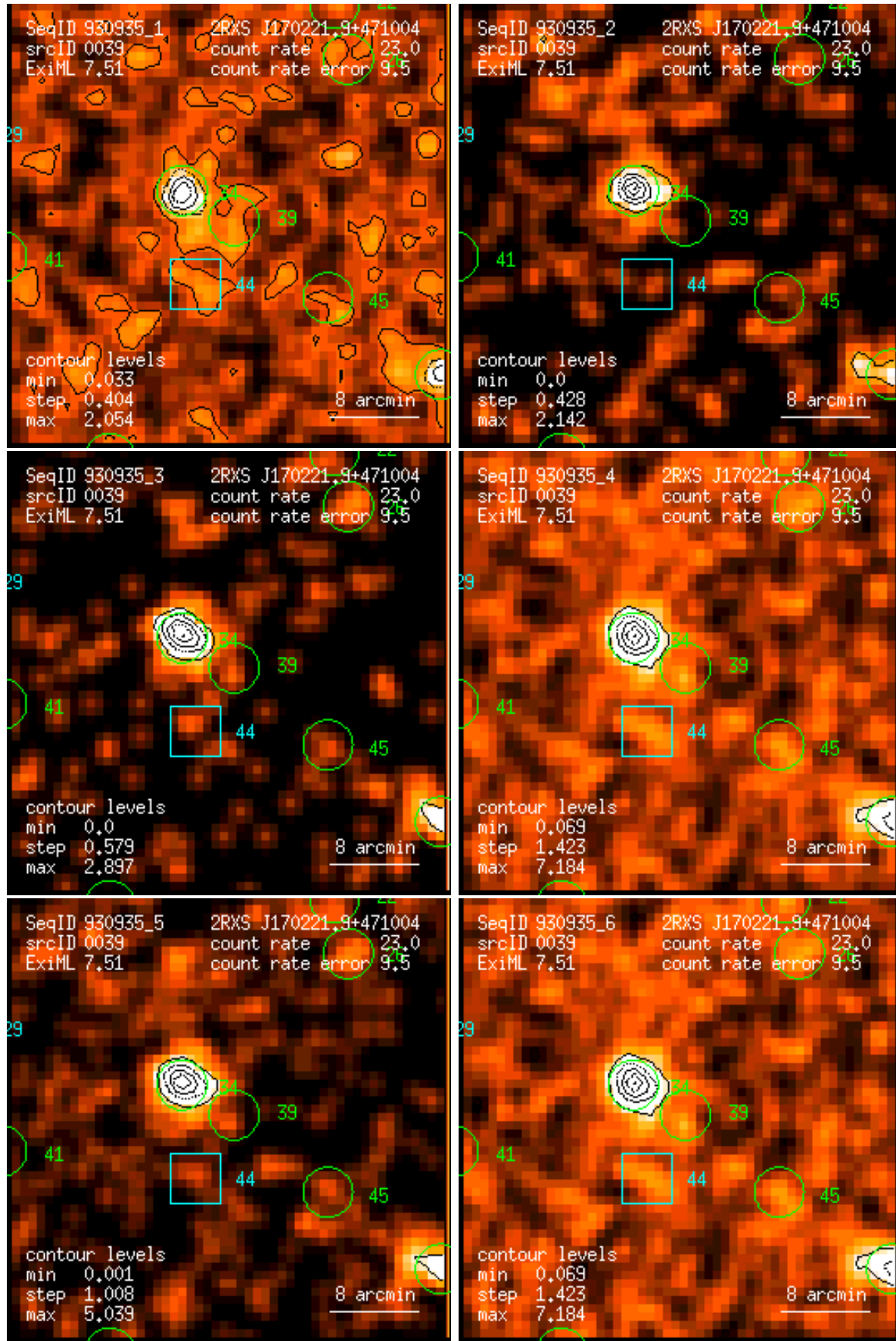
Figure 39: RASS 930935: detection 0039: band rate images, Gaussian filter: (1) PSPC channels 11 – 41, (2) 52 – 90, (3) 91 – 201, (4) 11 – 235, (5) 52 – 201, (6) 11 – 201. Broad band rates in counts/ks. Band rate contour levels in counts/ks/arcmin 2 .
