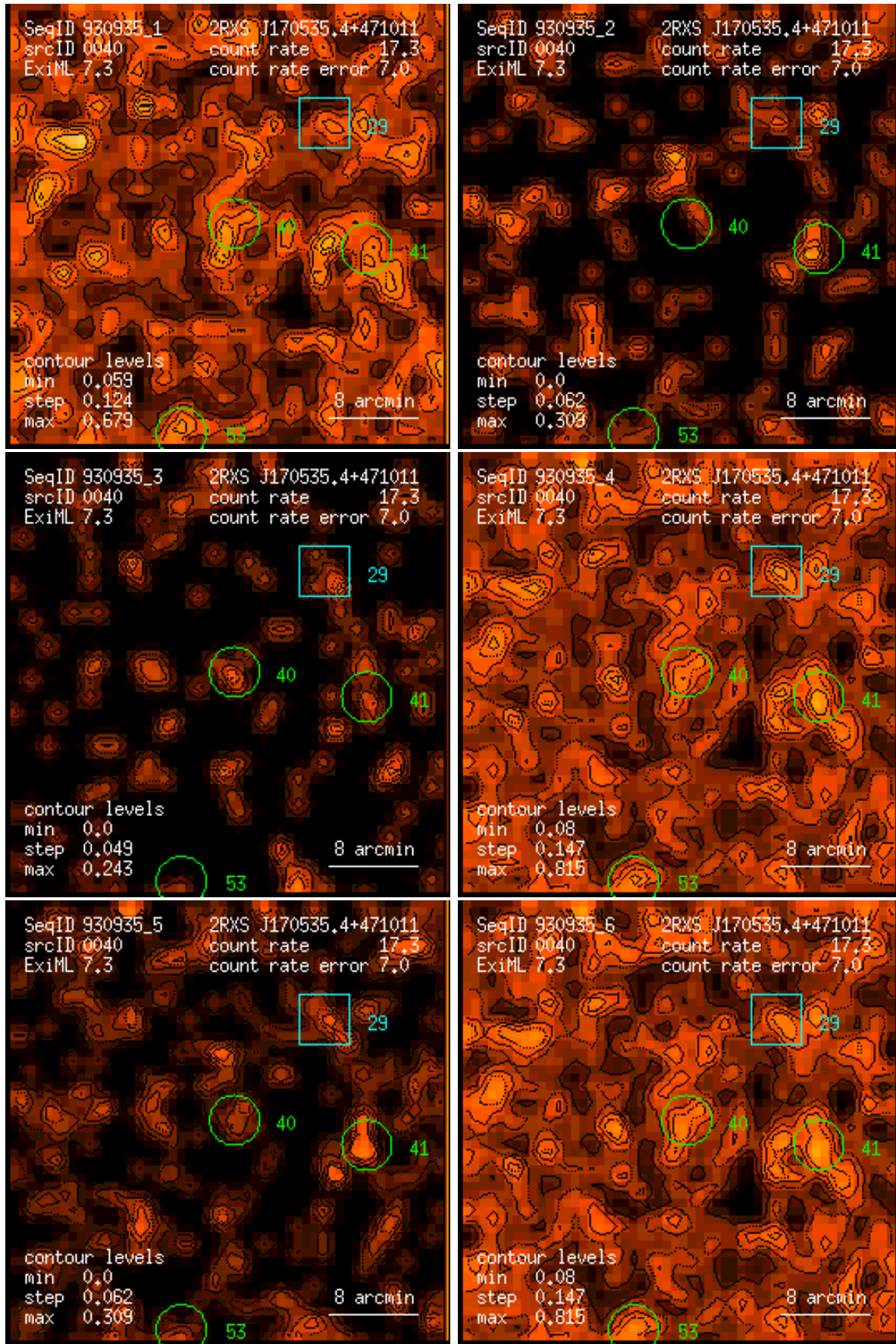
Figure 40: RASS 930935: detection 0040: band rate images, Gaussian filter: (1) PSPC channels 11 – 41, (2) 52 – 90, (3) 91 – 201, (4) 11 – 235, (5) 52 – 201, (6) 11 – 201. Broad band rates in counts/ks. Band rate contour levels in counts/ks/arcmin 2 .
