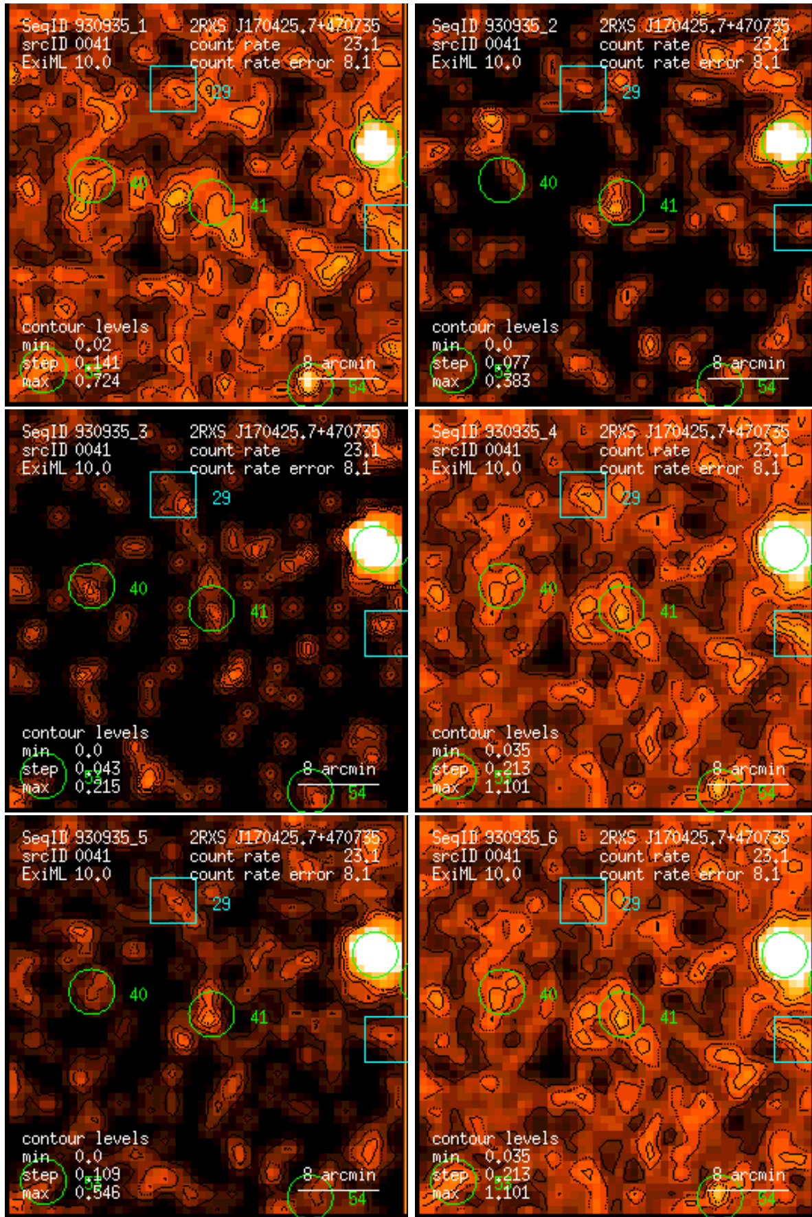
Figure 41: RASS 930935: detection 0041: band rate images, Gaussian filter: (1) PSPC channels 11 – 41, (2) 52 – 90, (3) 91 – 201, (4) 11 – 235, (5) 52 – 201, (6) 11 – 201. Broad band rates in counts/ks. Band rate contour levels in counts/ks/arcmin 2 .
