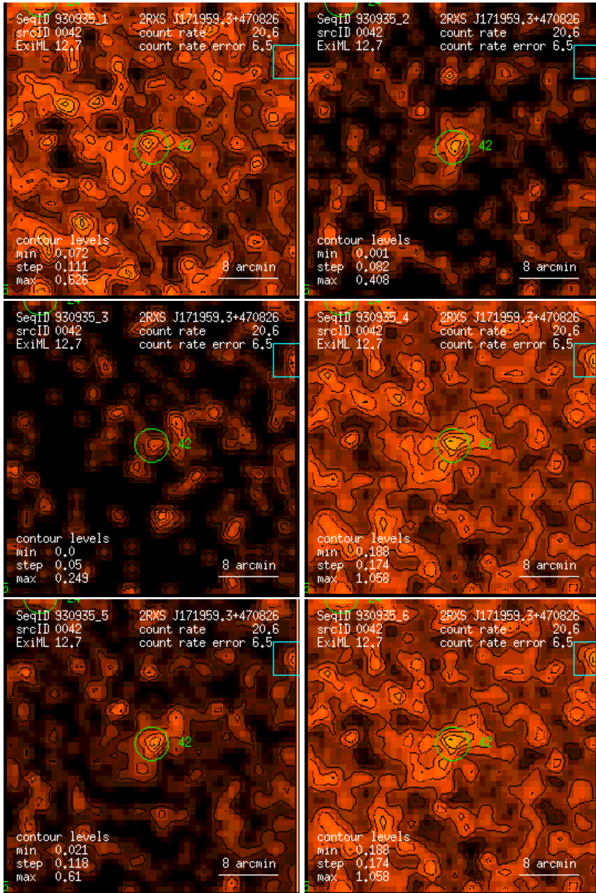
Figure 42: RASS 930935: detection 0042: band rate images, Gaussian filter: (1) PSPC channels 11 – 41, (2) 52 – 90, (3) 91 – 201, (4) 11 – 235, (5) 52 – 201, (6) 11 – 201. Broad band rates in counts/ks. Band rate contour levels in counts/ks/arcmin 2 .
