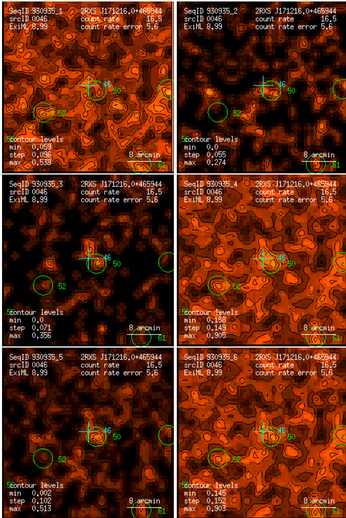
Figure 46: RASS 930935: detection 0046: band rate images, Gaussian filter: (1) PSPC channels 11 – 41, (2) 52 – 90, (3) 91 – 201, (4) 11 – 235, (5) 52 – 201, (6) 11 – 201. Broad band rates in counts/ks. Band rate contour levels in counts/ks/arcmin 2 .
