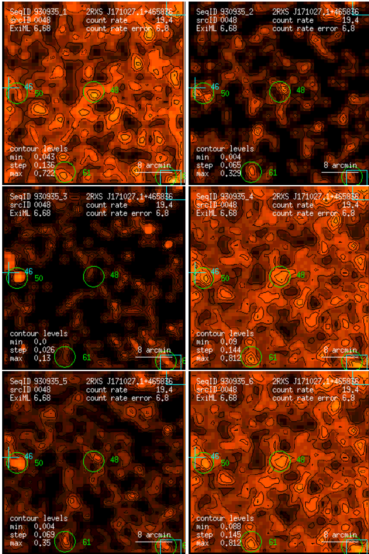
Figure 48: RASS 930935: detection 0048: band rate images, Gaussian filter: (1) PSPC channels 11 – 41, (2) 52 – 90, (3) 91 – 201, (4) 11 – 235, (5) 52 – 201, (6) 11 – 201. Broad band rates in counts/ks. Band rate contour levels in counts/ks/arcmin 2 .
