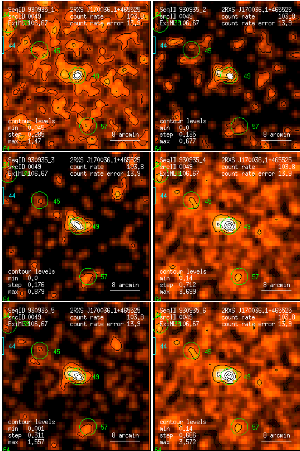
Figure 49: RASS 930935: detection 0049: band rate images, Gaussian filter: (1) PSPC channels 11 – 41, (2) 52 – 90, (3) 91 – 201, (4) 11 – 235, (5) 52 – 201, (6) 11 – 201. Broad band rates in counts/ks. Band rate contour levels in counts/ks/arcmin 2 .
