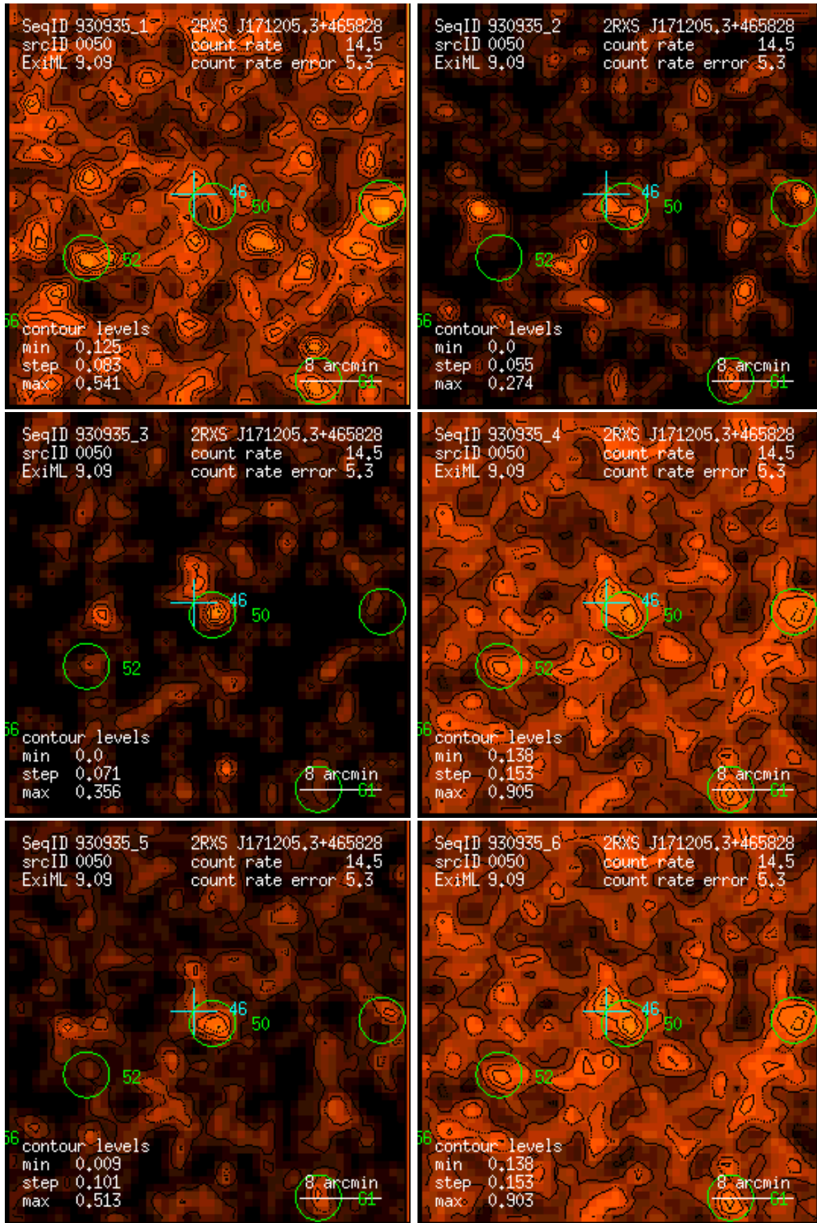
Figure 50: RASS 930935: detection 0050: band rate images, Gaussian filter: (1) PSPC channels 11 – 41, (2) 52 – 90, (3) 91 – 201, (4) 11 – 235, (5) 52 – 201, (6) 11 – 201. Broad band rates in counts/ks. Band rate contour levels in counts/ks/arcmin 2 .
