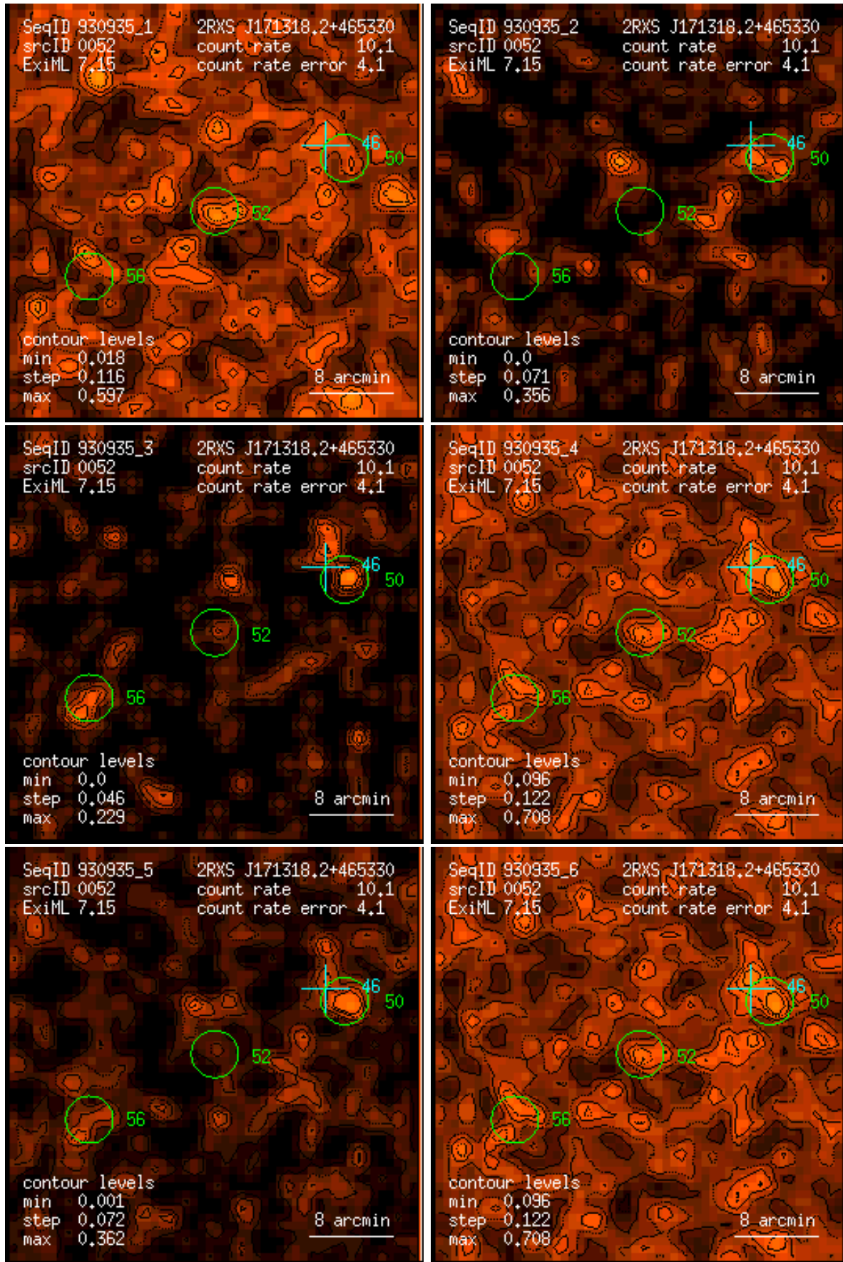
Figure 52: RASS 930935: detection 0052: band rate images, Gaussian filter: (1) PSPC channels 11 – 41, (2) 52 – 90, (3) 91 – 201, (4) 11 – 235, (5) 52 – 201, (6) 11 – 201. Broad band rates in counts/ks. Band rate contour levels in counts/ks/arcmin 2 .
