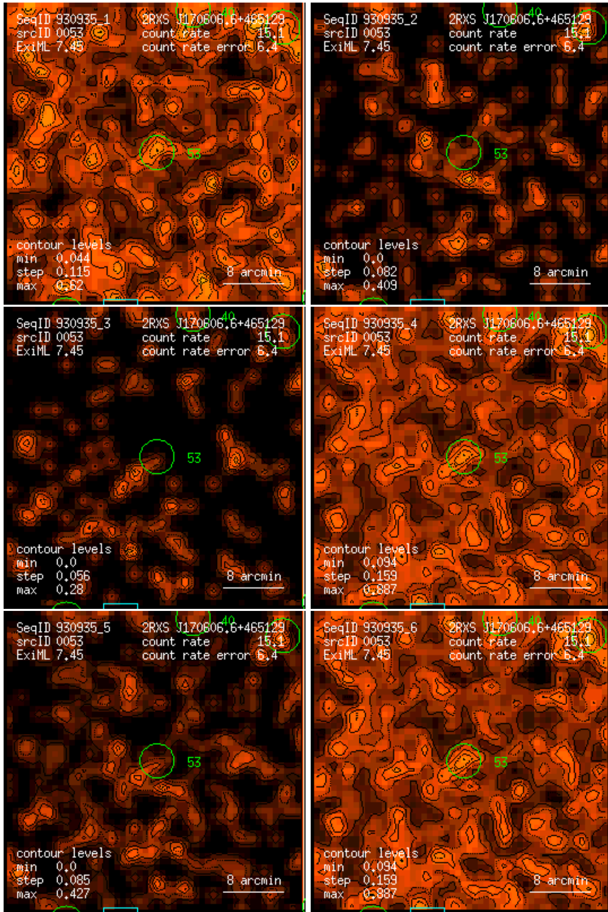
Figure 53: RASS 930935: detection 0053: band rate images, Gaussian filter: (1) PSPC channels 11 – 41, (2) 52 – 90, (3) 91 – 201, (4) 11 – 235, (5) 52 – 201, (6) 11 – 201. Broad band rates in counts/ks. Band rate contour levels in counts/ks/arcmin 2 .
