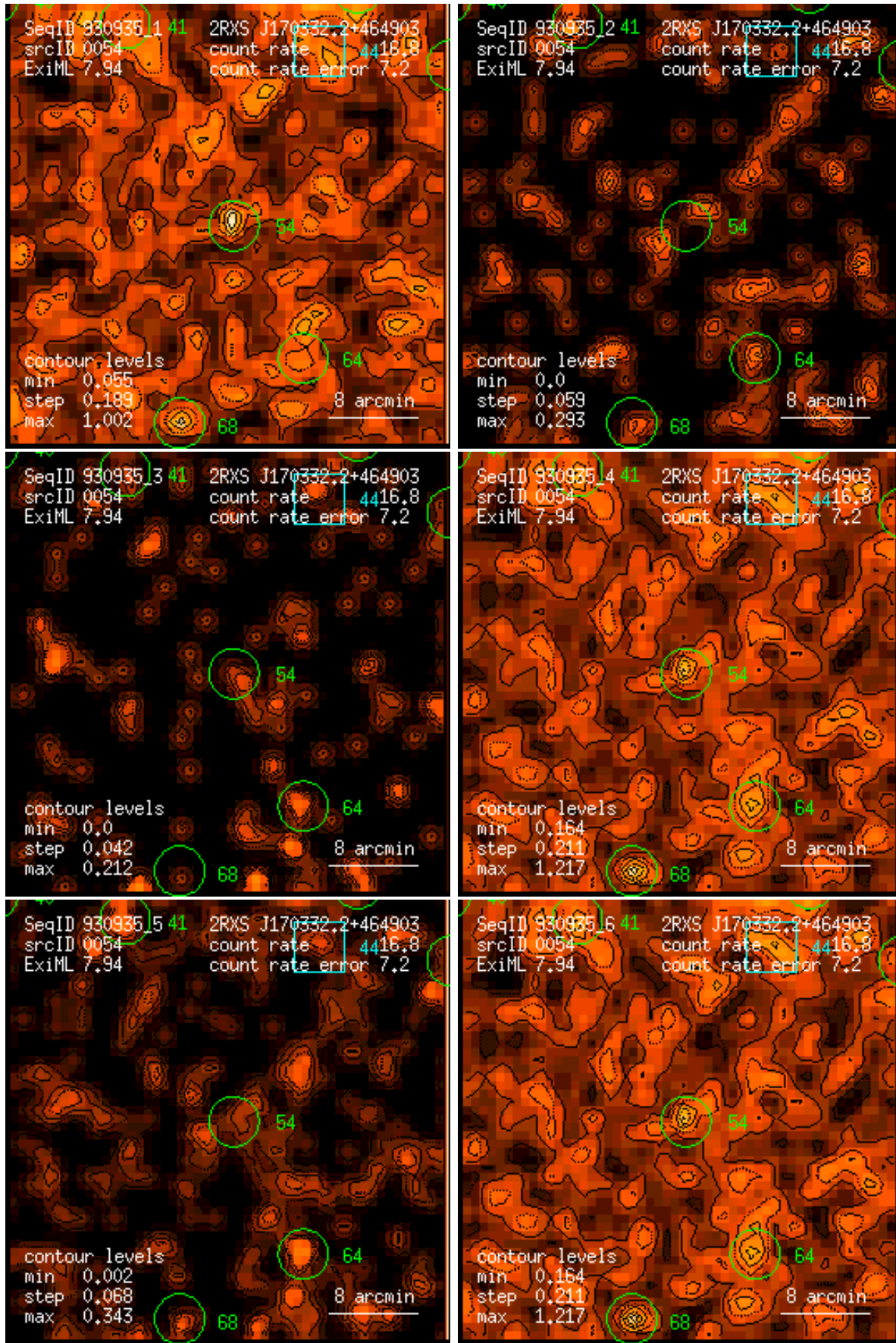
Figure 54: RASS 930935: detection 0054: band rate images, Gaussian filter: (1) PSPC channels 11 – 41, (2) 52 – 90, (3) 91 – 201, (4) 11 – 235, (5) 52 – 201, (6) 11 – 201. Broad band rates in counts/ks. Band rate contour levels in counts/ks/arcmin 2 .
