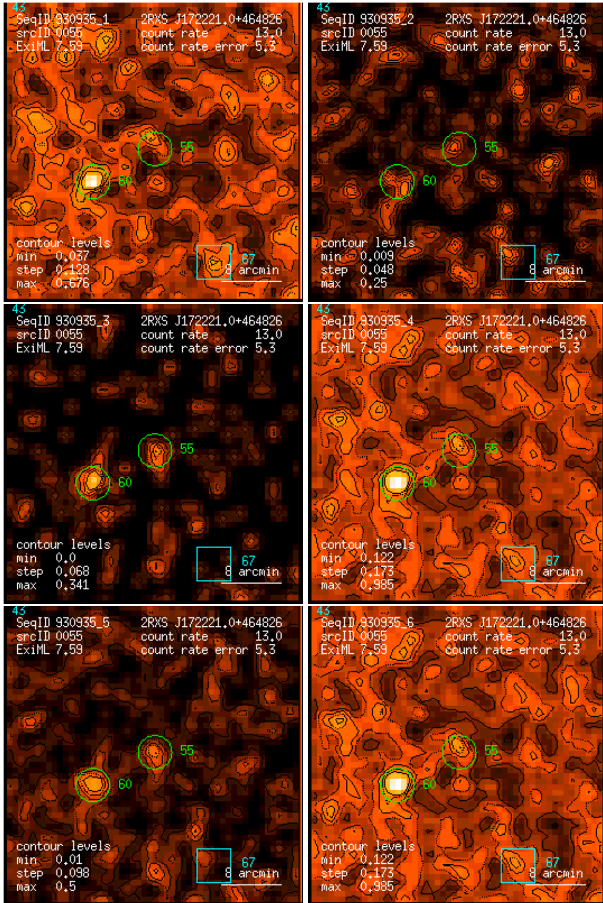
Figure 55: RASS 930935: detection 0055: band rate images, Gaussian filter: (1) PSPC channels 11 – 41, (2) 52 – 90, (3) 91 – 201, (4) 11 – 235, (5) 52 – 201, (6) 11 – 201. Broad band rates in counts/ks. Band rate contour levels in counts/ks/arcmin 2 .
