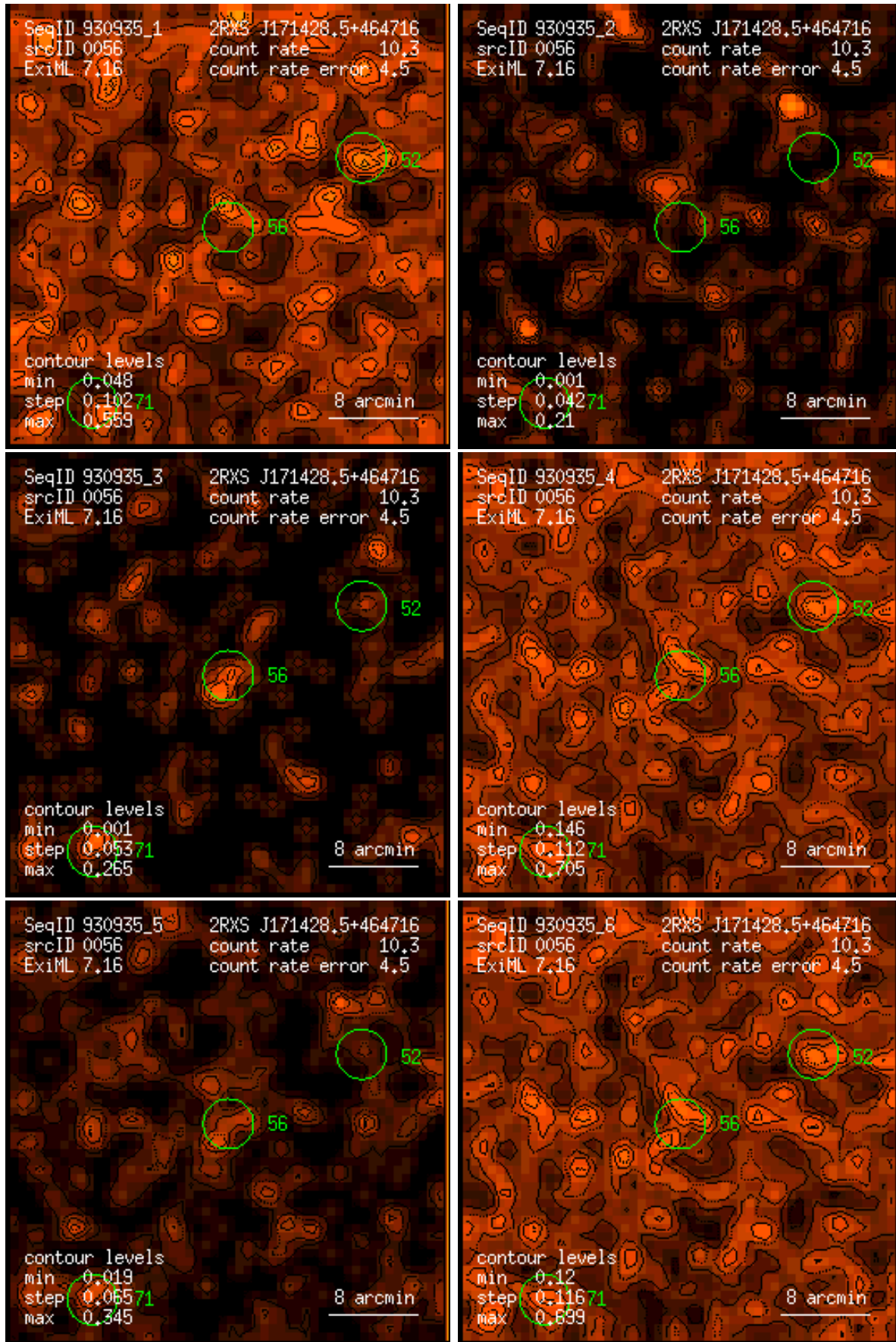
Figure 56: RASS 930935: detection 0056: band rate images, Gaussian filter: (1) PSPC channels 11 – 41, (2) 52 – 90, (3) 91 – 201, (4) 11 – 235, (5) 52 – 201, (6) 11 – 201. Broad band rates in counts/ks. Band rate contour levels in counts/ks/arcmin 2 .
