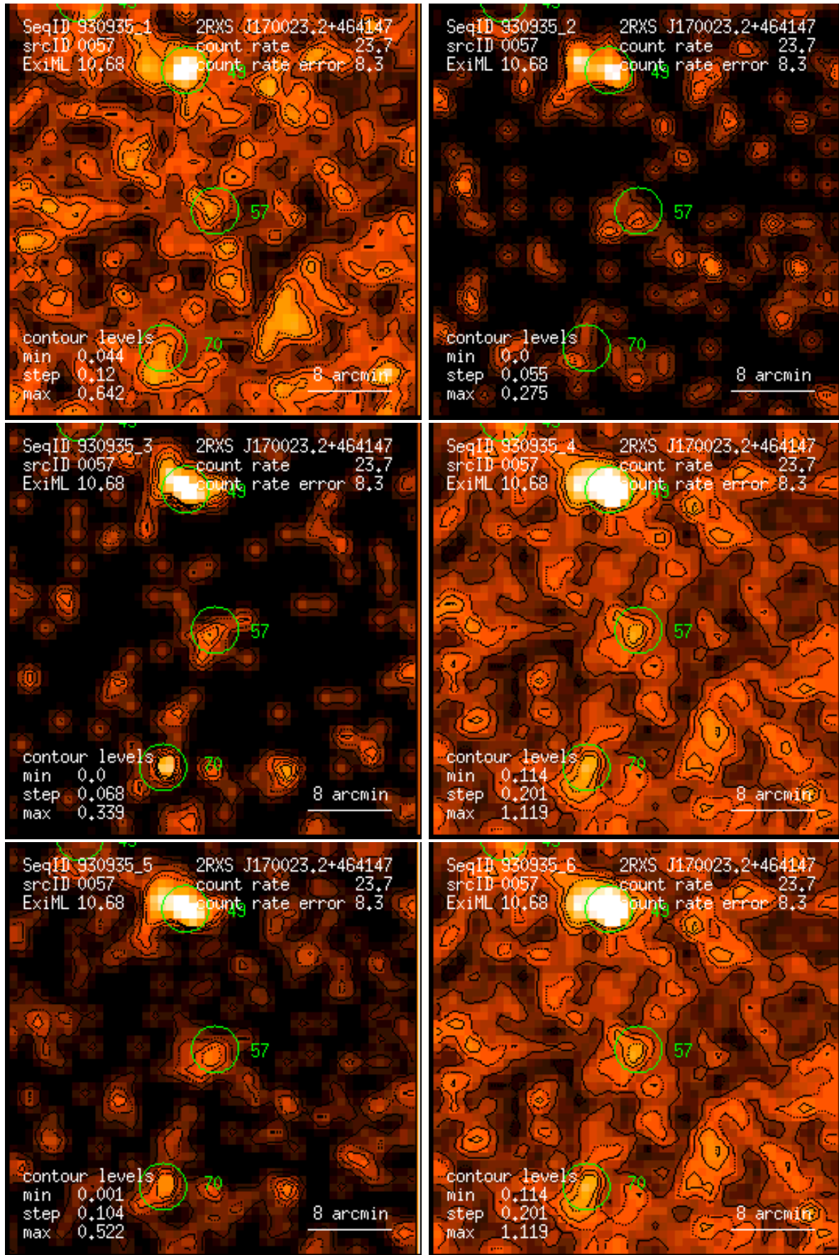
Figure 57: RASS 930935: detection 0057: band rate images, Gaussian filter: (1) PSPC channels 11 – 41, (2) 52 – 90, (3) 91 – 201, (4) 11 – 235, (5) 52 – 201, (6) 11 – 201. Broad band rates in counts/ks. Band rate contour levels in counts/ks/arcmin 2 .
