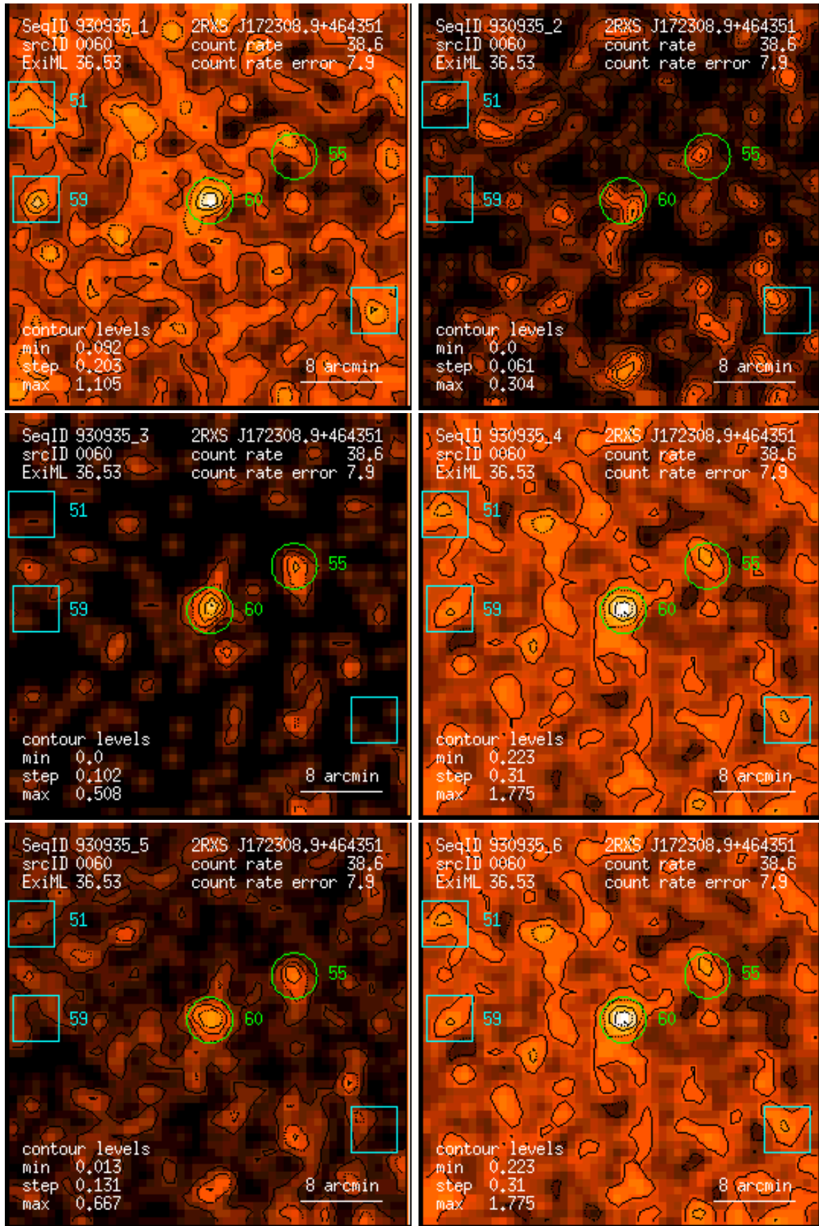
Figure 60: RASS 930935: detection 0060: band rate images, Gaussian filter: (1) PSPC channels 11 – 41, (2) 52 – 90, (3) 91 – 201, (4) 11 – 235, (5) 52 – 201, (6) 11 – 201. Broad band rates in counts/ks. Band rate contour levels in counts/ks/arcmin 2 .
