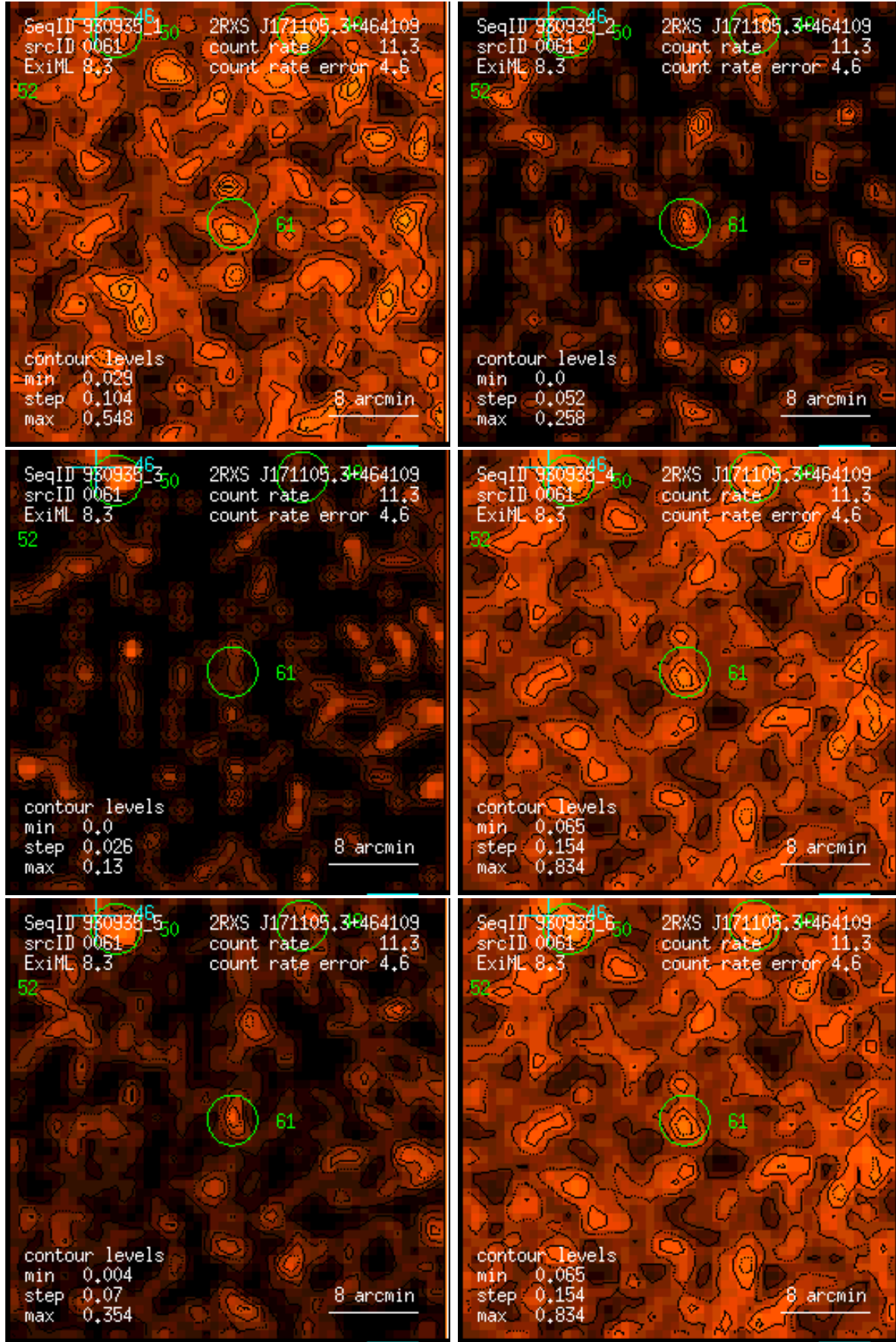
Figure 61: RASS 930935: detection 0061: band rate images, Gaussian filter: (1) PSPC channels 11 – 41, (2) 52 – 90, (3) 91 – 201, (4) 11 – 235, (5) 52 – 201, (6) 11 – 201. Broad band rates in counts/ks. Band rate contour levels in counts/ks/arcmin 2 .
