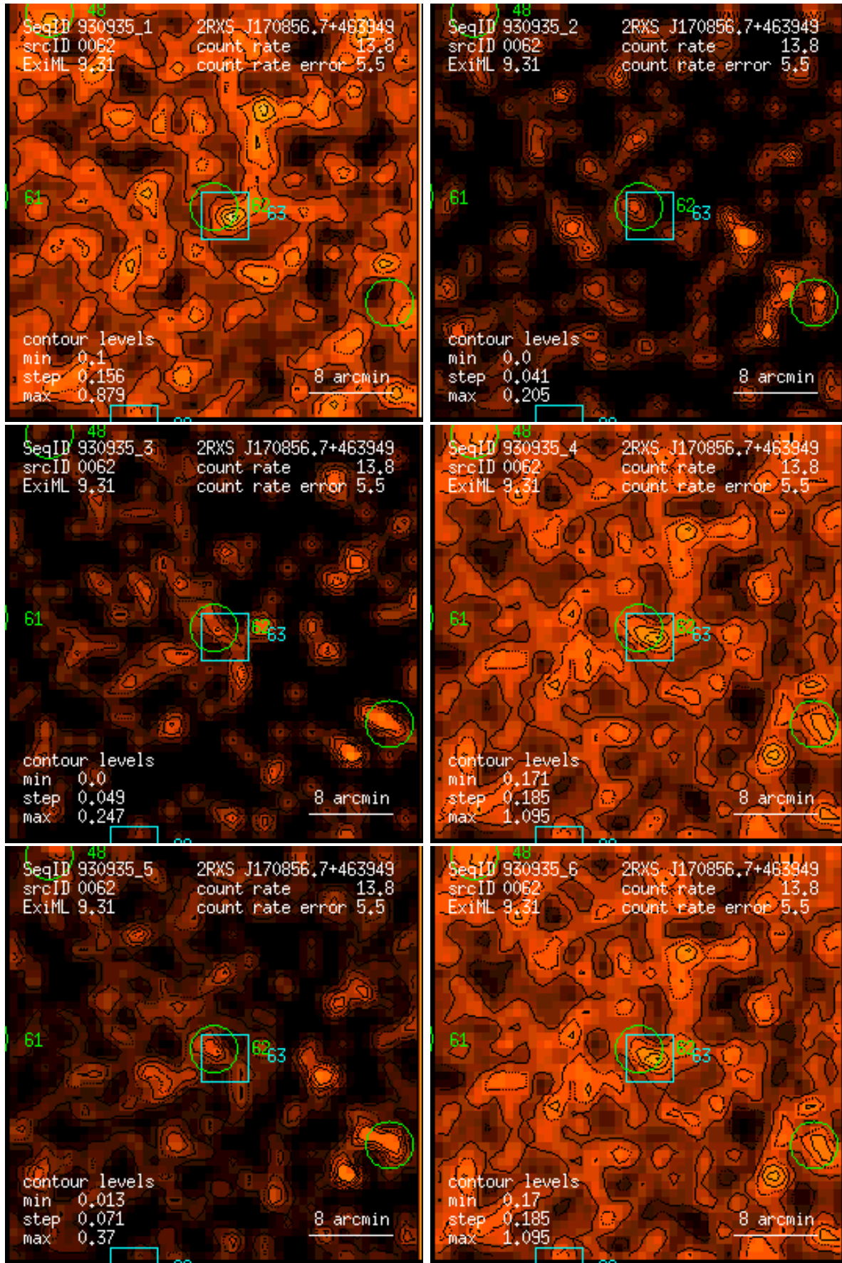
Figure 62: RASS 930935: detection 0062: band rate images, Gaussian filter: (1) PSPC channels 11 – 41, (2) 52 – 90, (3) 91 – 201, (4) 11 – 235, (5) 52 – 201, (6) 11 – 201. Broad band rates in counts/ks. Band rate contour levels in counts/ks/arcmin 2 .
