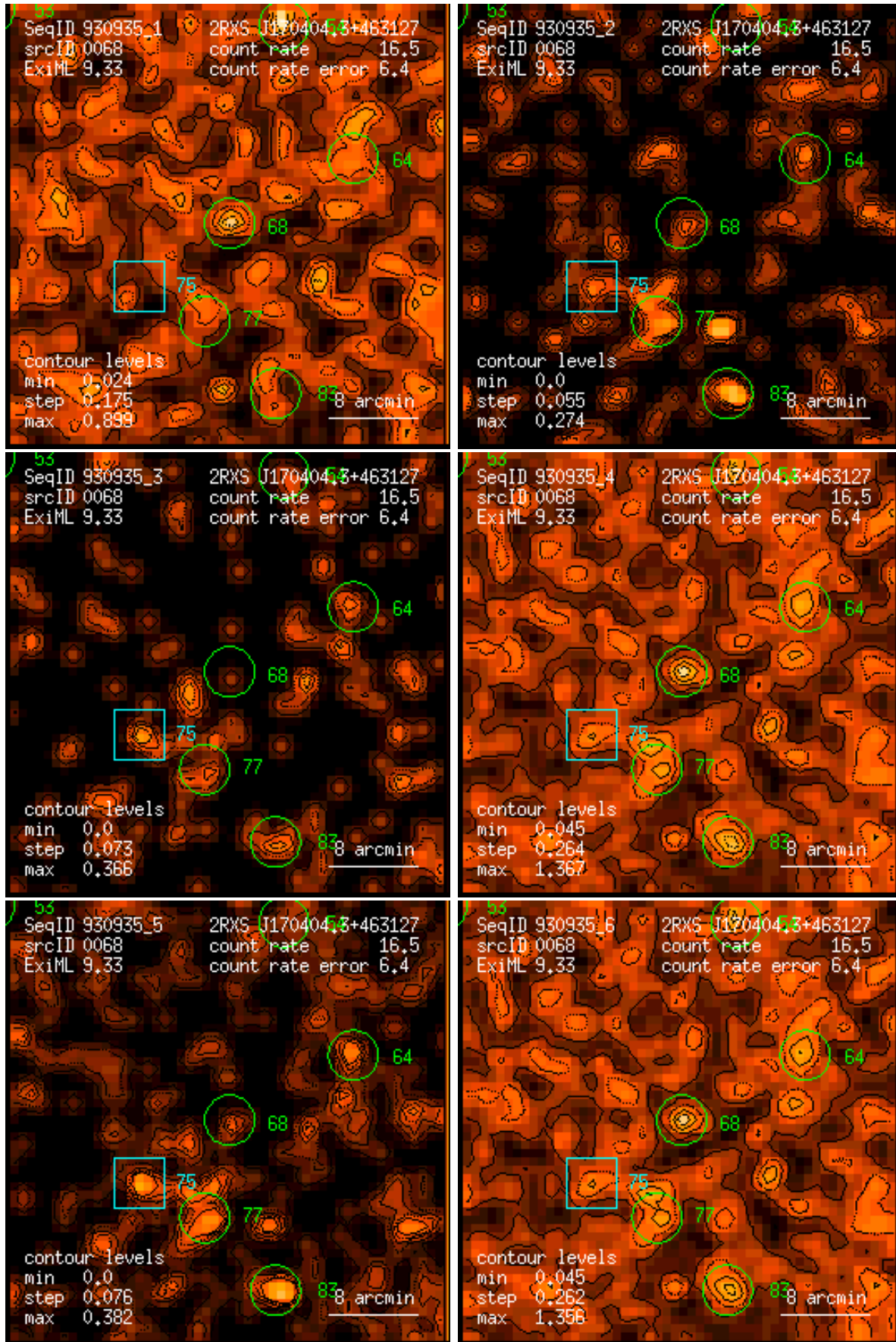
Figure 68: RASS 930935: detection 0068: band rate images, Gaussian filter: (1) PSPC channels 11 – 41, (2) 52 – 90, (3) 91 – 201, (4) 11 – 235, (5) 52 – 201, (6) 11 – 201. Broad band rates in counts/ks. Band rate contour levels in counts/ks/arcmin 2 .
