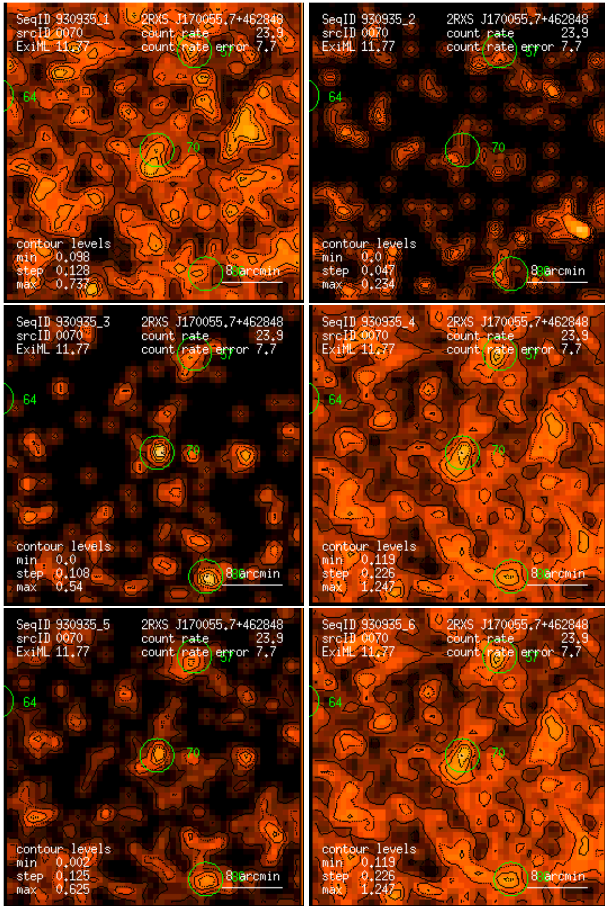
Figure 70: RASS 930935: detection 0070: band rate images, Gaussian filter: (1) PSPC channels 11 – 41, (2) 52 – 90, (3) 91 – 201, (4) 11 – 235, (5) 52 – 201, (6) 11 – 201. Broad band rates in counts/ks. Band rate contour levels in counts/ks/arcmin 2 .
