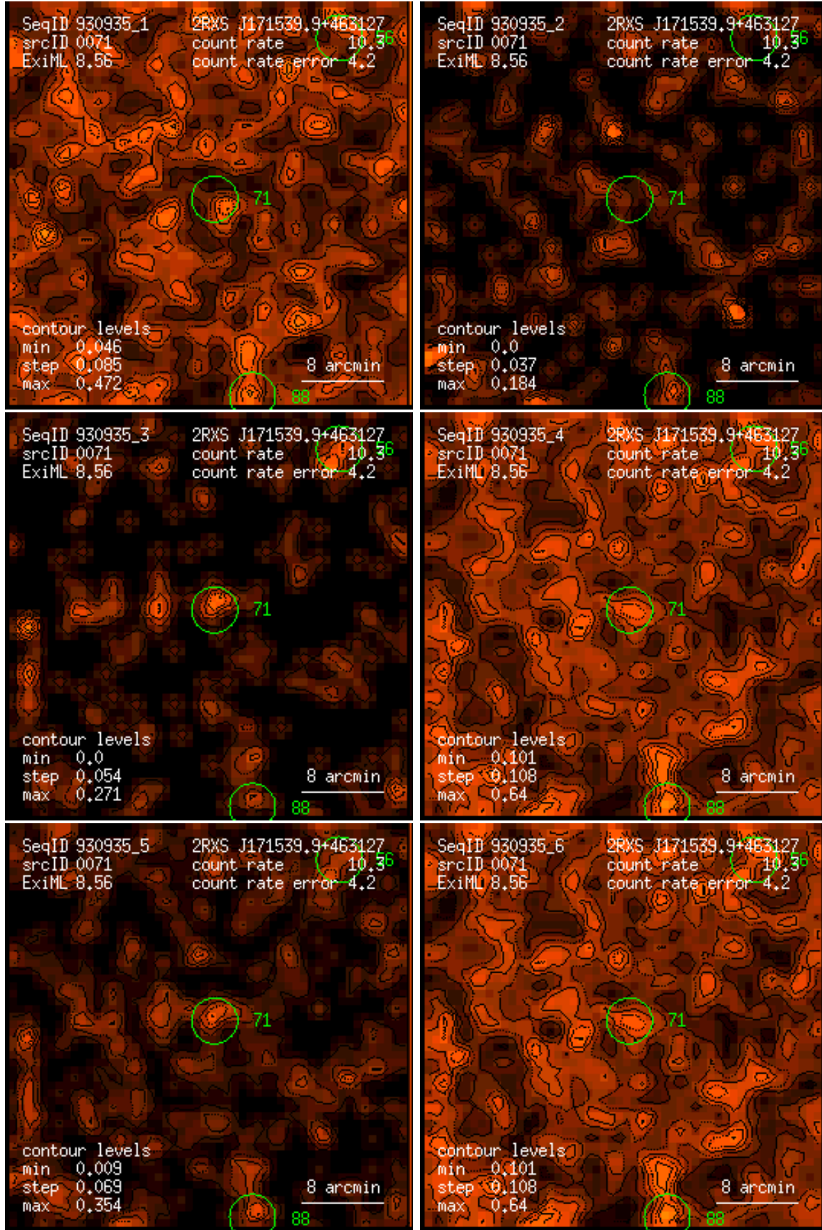
Figure 71: RASS 930935: detection 0071: band rate images, Gaussian filter: (1) PSPC channels 11 – 41, (2) 52 – 90, (3) 91 – 201, (4) 11 – 235, (5) 52 – 201, (6) 11 – 201. Broad band rates in counts/ks. Band rate contour levels in counts/ks/arcmin 2 .
