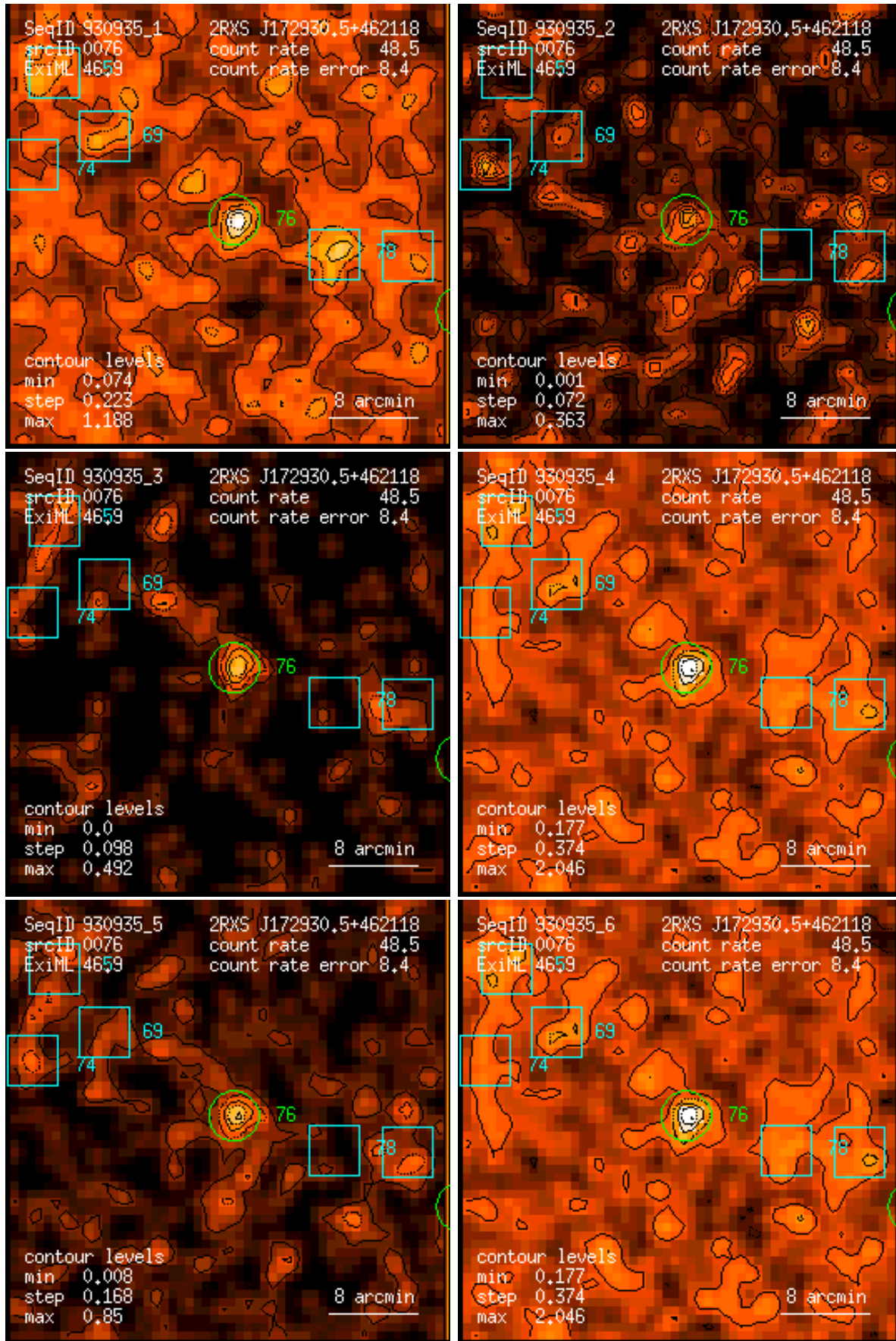
Figure 76: RASS 930935: detection 0076: band rate images, Gaussian filter: (1) PSPC channels 11 – 41, (2) 52 – 90, (3) 91 – 201, (4) 11 – 235, (5) 52 – 201, (6) 11 – 201. Broad band rates in counts/ks. Band rate contour levels in counts/ks/arcmin 2 .
