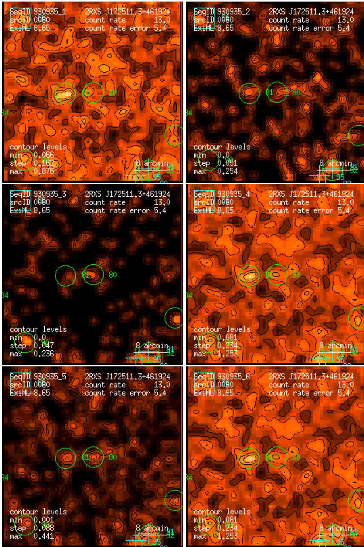
Figure 80: RASS 930935: detection 0080: band rate images, Gaussian filter: (1) PSPC channels 11 – 41, (2) 52 – 90, (3) 91 – 201, (4) 11 – 235, (5) 52 – 201, (6) 11 – 201. Broad band rates in counts/ks. Band rate contour levels in counts/ks/arcmin 2 .
