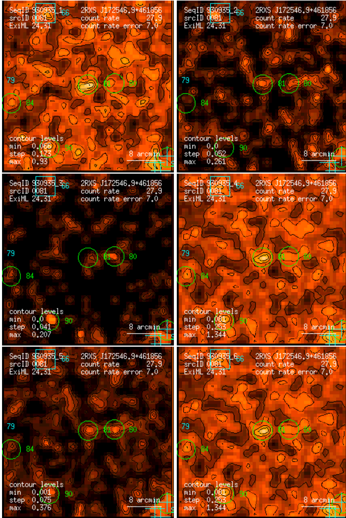
Figure 81: RASS 930935: detection 0081: band rate images, Gaussian filter: (1) PSPC channels 11 – 41, (2) 52 – 90, (3) 91 – 201, (4) 11 – 235, (5) 52 – 201, (6) 11 – 201. Broad band rates in counts/ks. Band rate contour levels in counts/ks/arcmin 2 .
