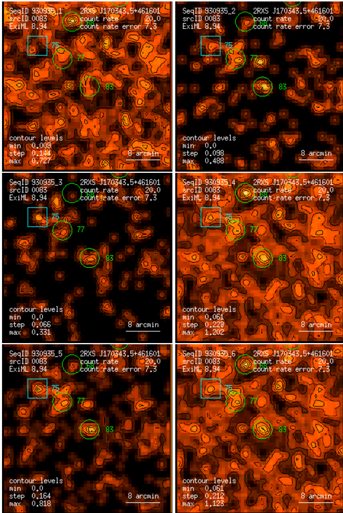
Figure 83: RASS 930935: detection 0083: band rate images, Gaussian filter: (1) PSPC channels 11 – 41, (2) 52 – 90, (3) 91 – 201, (4) 11 – 235, (5) 52 – 201, (6) 11 – 201. Broad band rates in counts/ks. Band rate contour levels in counts/ks/arcmin 2 .
