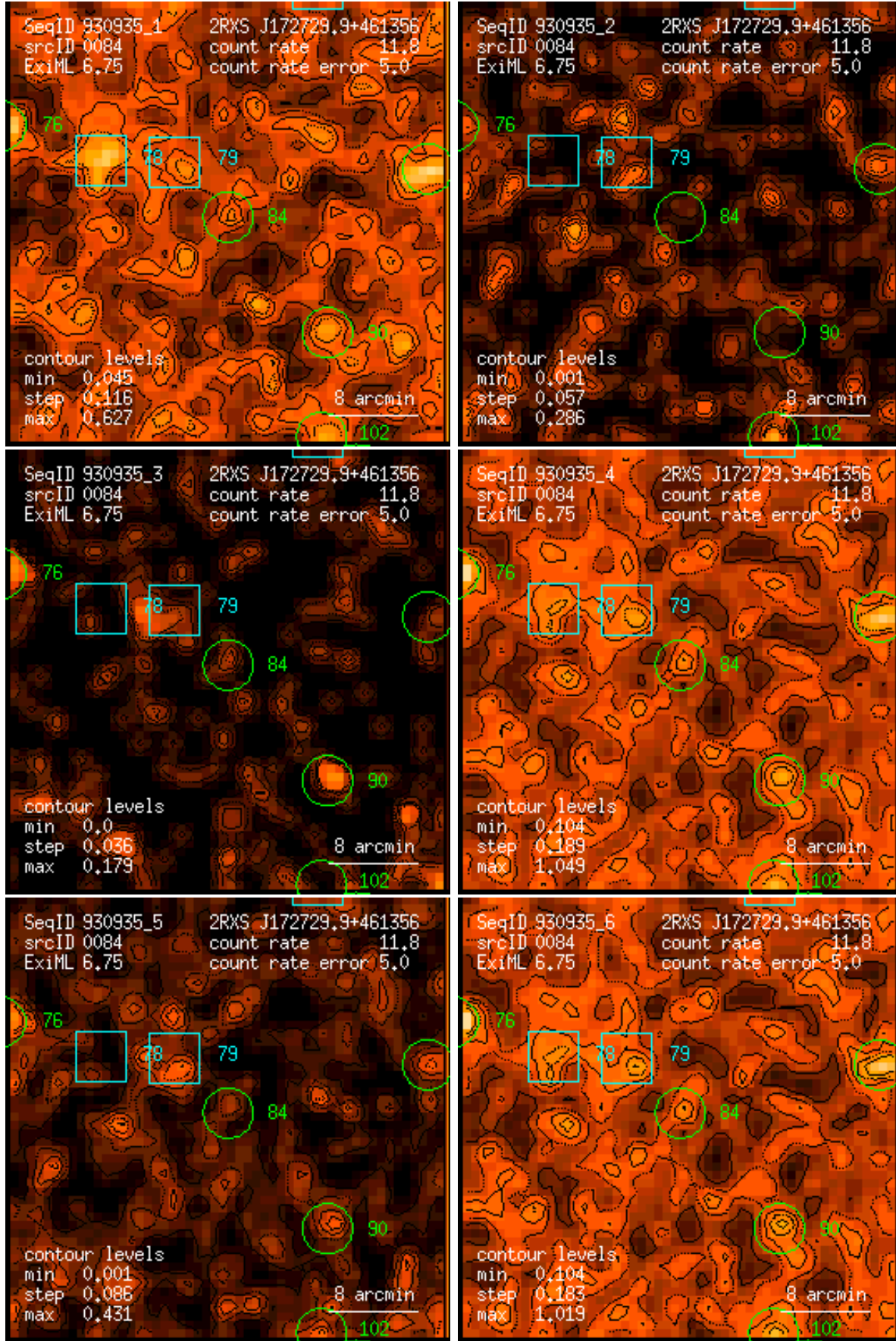
Figure 84: RASS 930935: detection 0084: band rate images, Gaussian filter: (1) PSPC channels 11 – 41, (2) 52 – 90, (3) 91 – 201, (4) 11 – 235, (5) 52 – 201, (6) 11 – 201. Broad band rates in counts/ks. Band rate contour levels in counts/ks/arcmin 2 .
