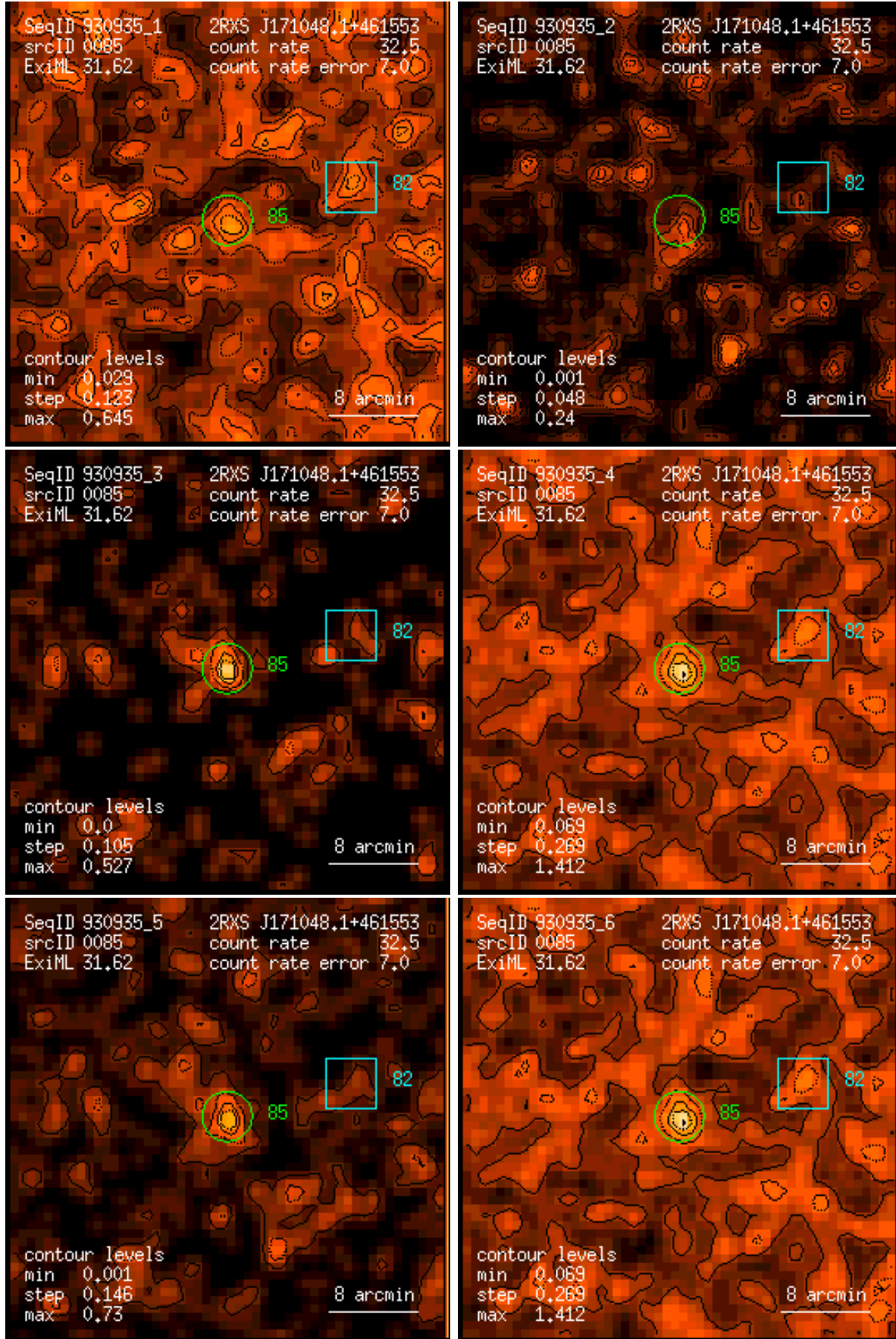
Figure 85: RASS 930935: detection 0085: band rate images, Gaussian filter: (1) PSPC channels 11 – 41, (2) 52 – 90, (3) 91 – 201, (4) 11 – 235, (5) 52 – 201, (6) 11 – 201. Broad band rates in counts/ks. Band rate contour levels in counts/ks/arcmin 2 .
