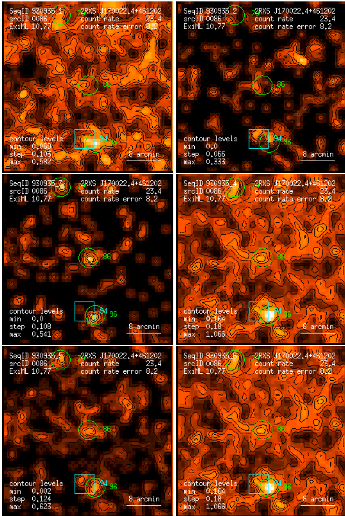
Figure 86: RASS 930935: detection 0086: band rate images, Gaussian filter: (1) PSPC channels 11 – 41, (2) 52 – 90, (3) 91 – 201, (4) 11 – 235, (5) 52 – 201, (6) 11 – 201. Broad band rates in counts/ks. Band rate contour levels in counts/ks/arcmin 2 .
