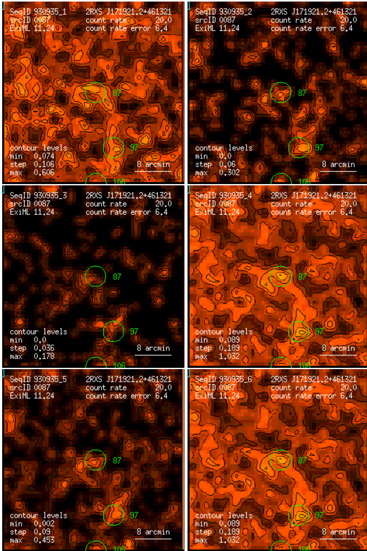
Figure 87: RASS 930935: detection 0087: band rate images, Gaussian filter: (1) PSPC channels 11 – 41, (2) 52 – 90, (3) 91 – 201, (4) 11 – 235, (5) 52 – 201, (6) 11 – 201. Broad band rates in counts/ks. Band rate contour levels in counts/ks/arcmin 2 .
