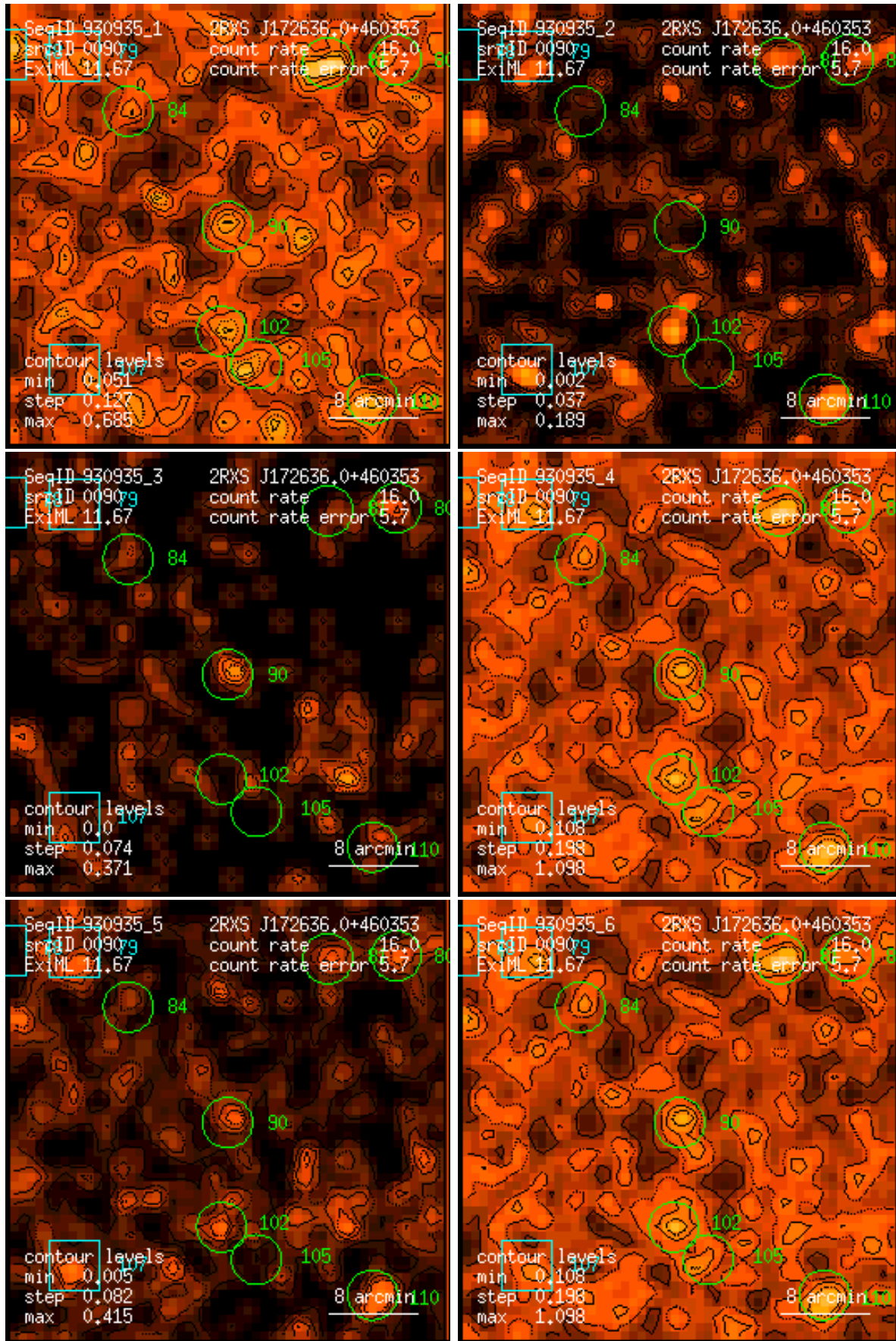
Figure 90: RASS 930935: detection 0090: band rate images, Gaussian filter: (1) PSPC channels 11 – 41, (2) 52 – 90, (3) 91 – 201, (4) 11 – 235, (5) 52 – 201, (6) 11 – 201. Broad band rates in counts/ks. Band rate contour levels in counts/ks/arcmin 2 .
