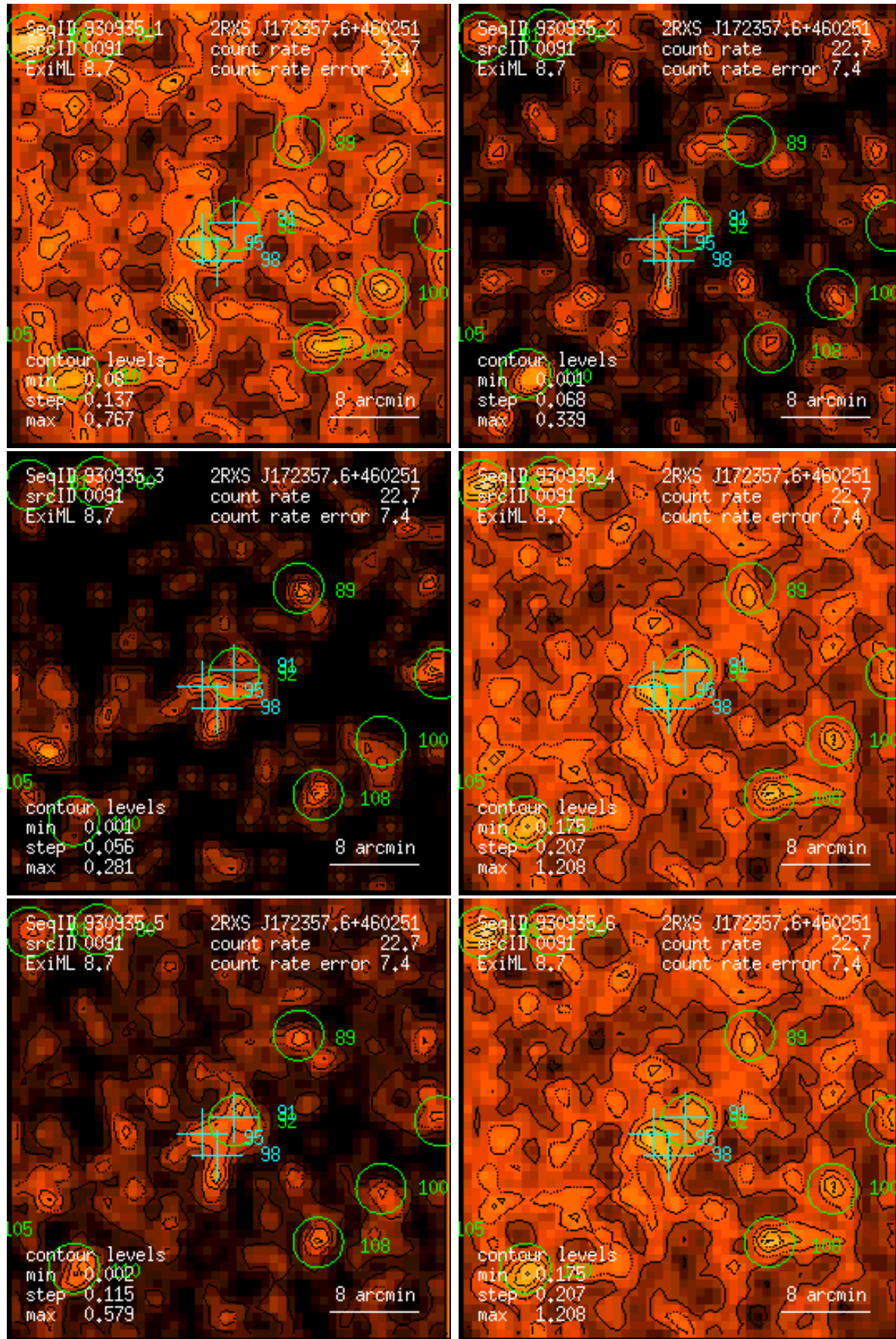
Figure 91: RASS 930935: detection 0091: band rate images, Gaussian filter: (1) PSPC channels 11 – 41, (2) 52 – 90, (3) 91 – 201, (4) 11 – 235, (5) 52 – 201, (6) 11 – 201. Broad band rates in counts/ks. Band rate contour levels in counts/ks/arcmin 2 .
