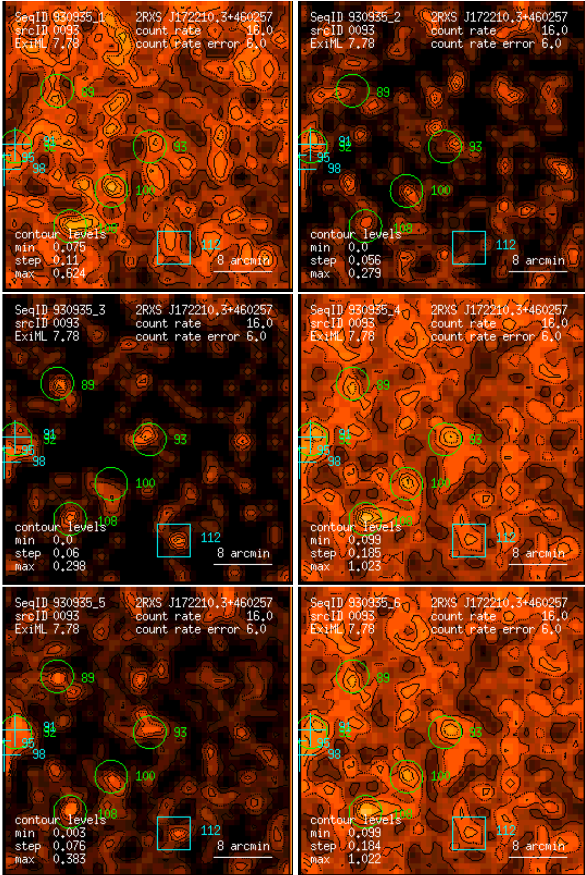
Figure 93: RASS 930935: detection 0093: band rate images, Gaussian filter: (1) PSPC channels 11 – 41, (2) 52 – 90, (3) 91 – 201, (4) 11 – 235, (5) 52 – 201, (6) 11 – 201. Broad band rates in counts/ks. Band rate contour levels in counts/ks/arcmin 2 .
