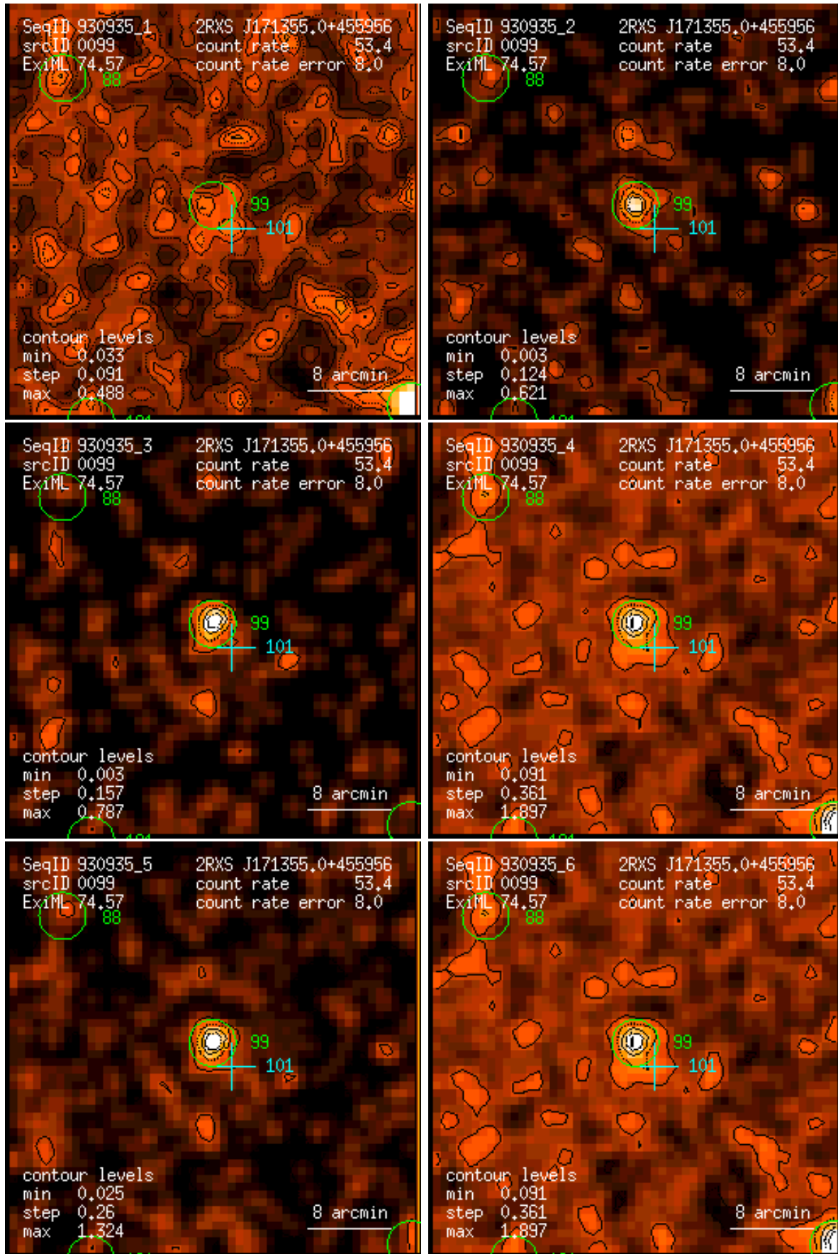
Figure 99: RASS 930935: detection 0099: band rate images, Gaussian filter: (1) PSPC channels 11 – 41, (2) 52 – 90, (3) 91 – 201, (4) 11 – 235, (5) 52 – 201, (6) 11 – 201. Broad band rates in counts/ks. Band rate contour levels in counts/ks/arcmin 2 .
