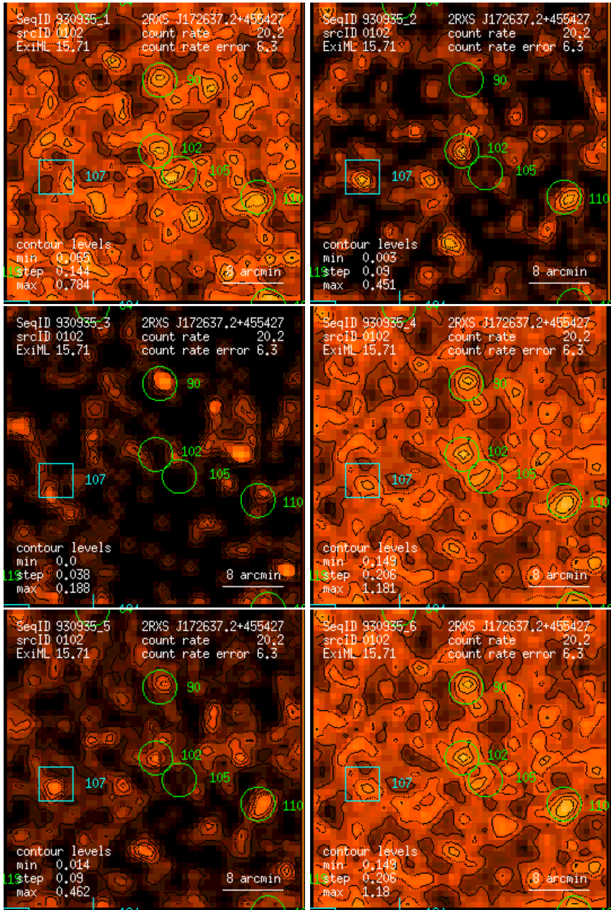
Figure 102: RASS 930935: detection 0102: band rate images, Gaussian filter: (1) PSPC channels 11 – 41, (2) 52 – 90, (3) 91 – 201, (4) 11 – 235, (5) 52 – 201, (6) 11 – 201. Broad band rates in counts/ks. Band rate contour levels in counts/ks/arcmin 2 .
