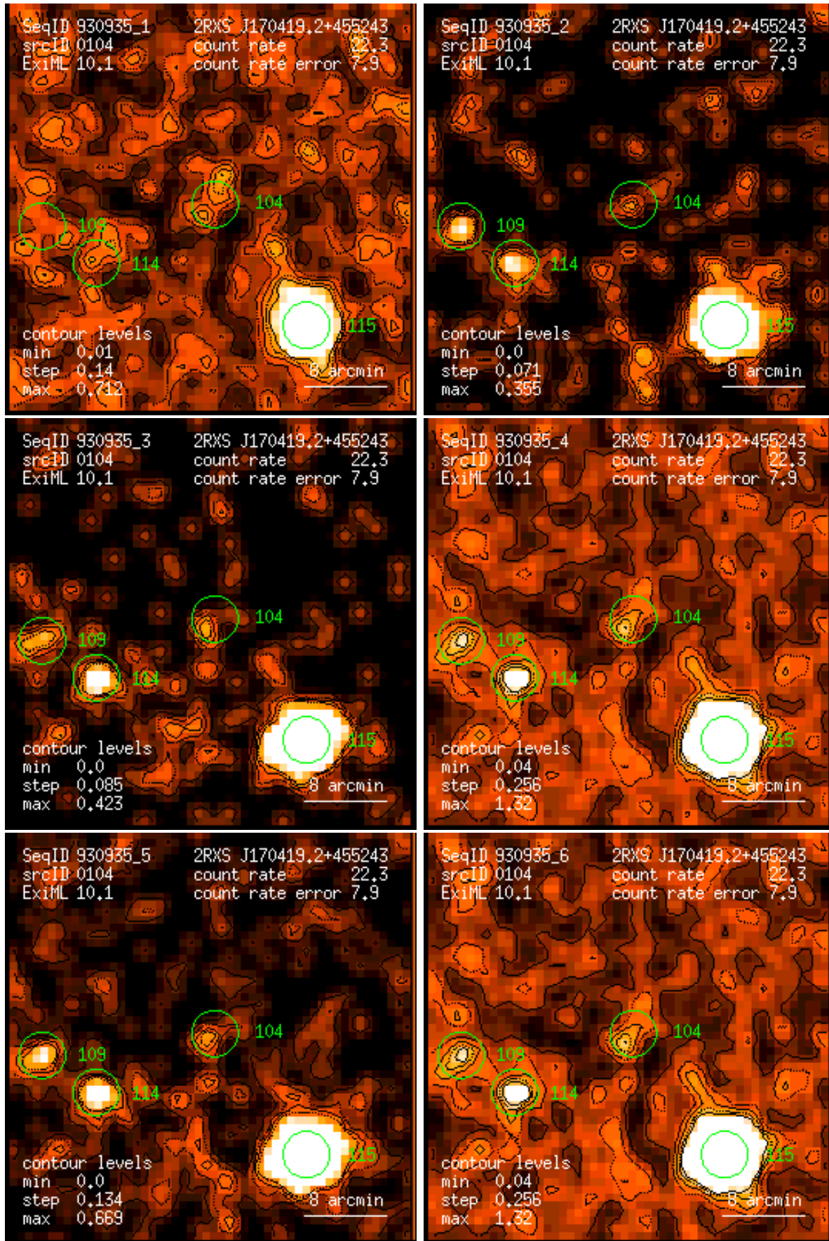
Figure 104: RASS 930935: detection 0104: band rate images, Gaussian filter: (1) PSPC channels 11 – 41, (2) 52 – 90, (3) 91 – 201, (4) 11 – 235, (5) 52 – 201, (6) 11 – 201. Broad band rates in counts/ks. Band rate contour levels in counts/ks/arcmin 2 .
