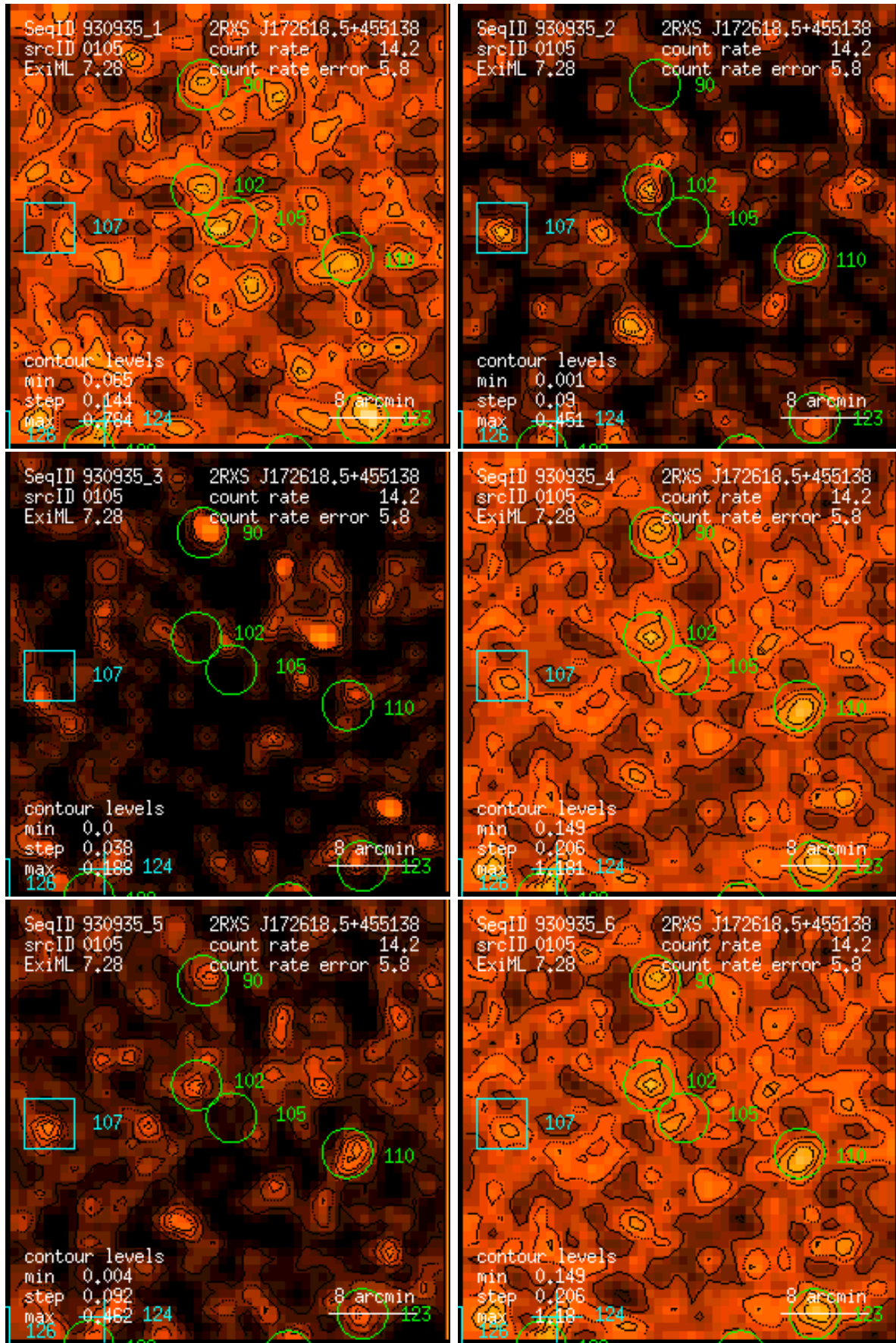
Figure 105: RASS 930935: detection 0105: band rate images, Gaussian filter: (1) PSPC channels 11 – 41, (2) 52 – 90, (3) 91 – 201, (4) 11 – 235, (5) 52 – 201, (6) 11 – 201. Broad band rates in counts/ks. Band rate contour levels in counts/ks/arcmin 2 .
