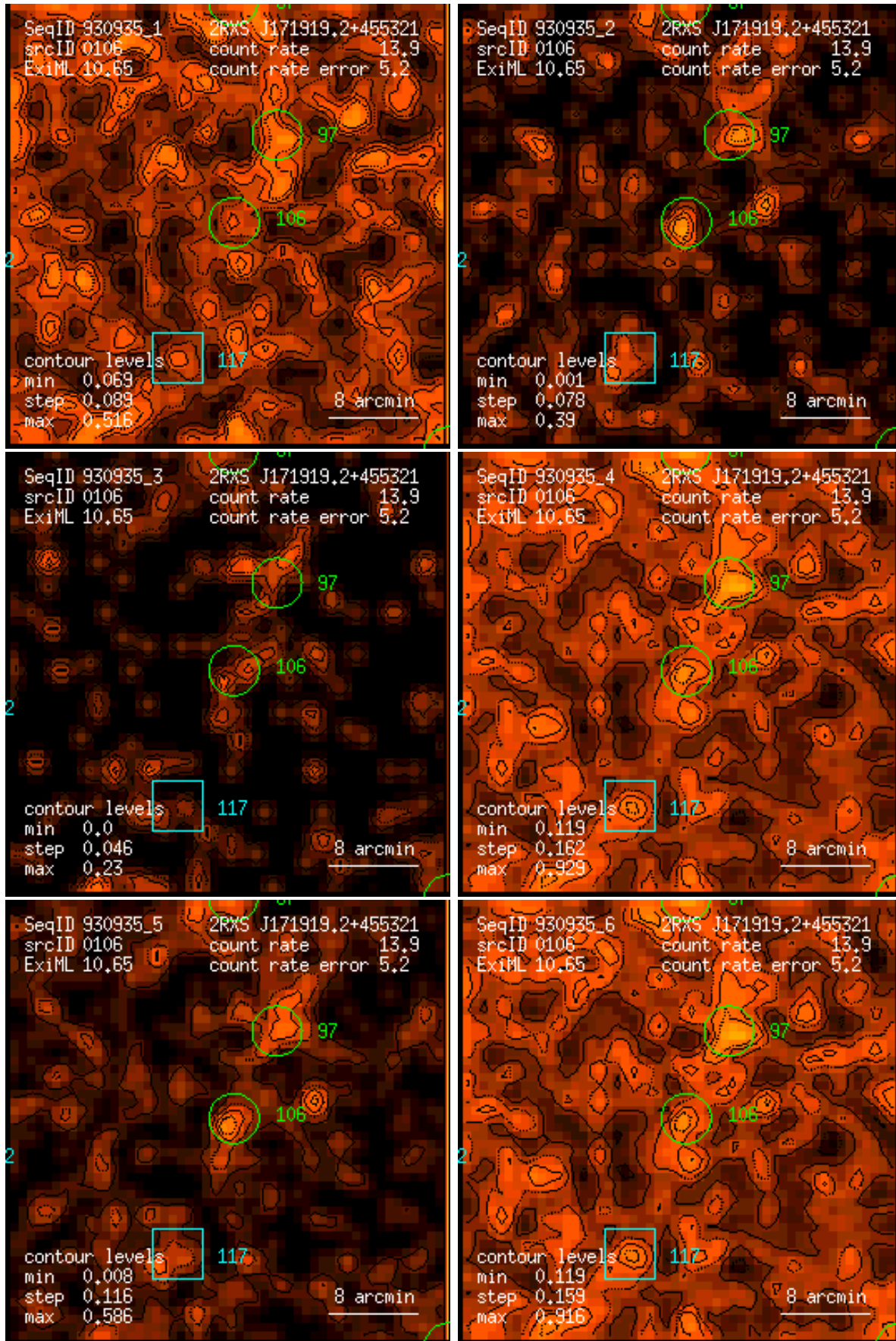
Figure 106: RASS 930935: detection 0106: band rate images, Gaussian filter: (1) PSPC channels 11 – 41, (2) 52 – 90, (3) 91 – 201, (4) 11 – 235, (5) 52 – 201, (6) 11 – 201. Broad band rates in counts/ks. Band rate contour levels in counts/ks/arcmin 2 .
