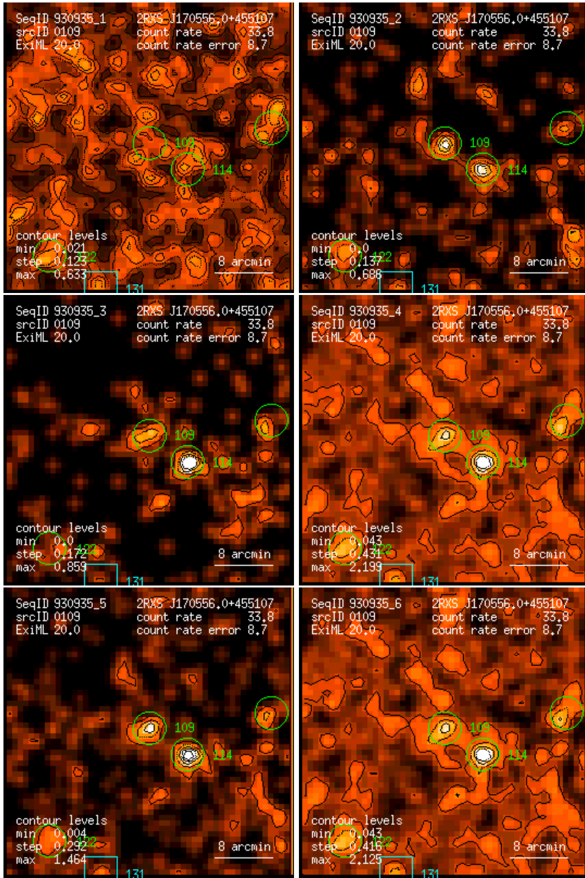
Figure 109: RASS 930935: detection 0109: band rate images, Gaussian filter: (1) PSPC channels 11 – 41, (2) 52 – 90, (3) 91 – 201, (4) 11 – 235, (5) 52 – 201, (6) 11 – 201. Broad band rates in counts/ks. Band rate contour levels in counts/ks/arcmin 2 .
