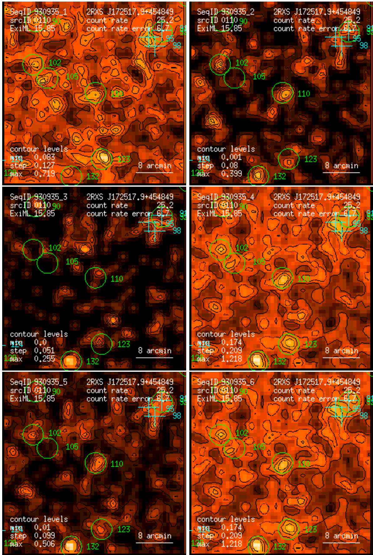
Figure 110: RASS 930935: detection 0110: band rate images, Gaussian filter: (1) PSPC channels 11 – 41, (2) 52 – 90, (3) 91 – 201, (4) 11 – 235, (5) 52 – 201, (6) 11 – 201. Broad band rates in counts/ks. Band rate contour levels in counts/ks/arcmin 2 .
