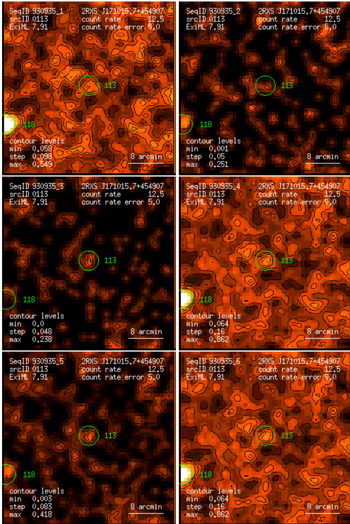
Figure 113: RASS 930935: detection 0113: band rate images, Gaussian filter: (1) PSPC channels 11 – 41, (2) 52 – 90, (3) 91 – 201, (4) 11 – 235, (5) 52 – 201, (6) 11 – 201. Broad band rates in counts/ks. Band rate contour levels in counts/ks/arcmin 2 .
