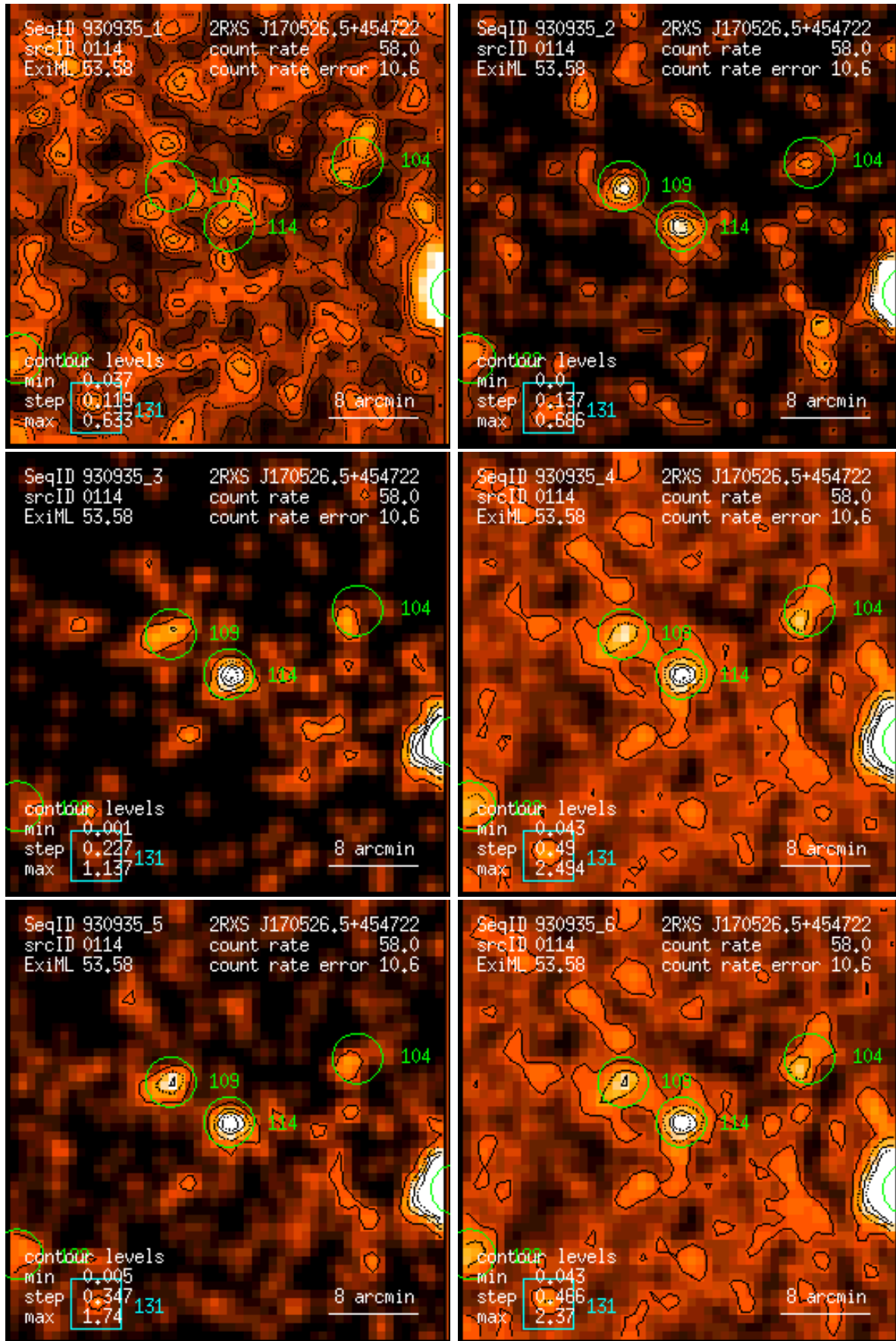
Figure 114: RASS 930935: detection 0114: band rate images, Gaussian filter: (1) PSPC channels 11 – 41, (2) 52 – 90, (3) 91 – 201, (4) 11 – 235, (5) 52 – 201, (6) 11 – 201. Broad band rates in counts/ks. Band rate contour levels in counts/ks/arcmin 2 .
