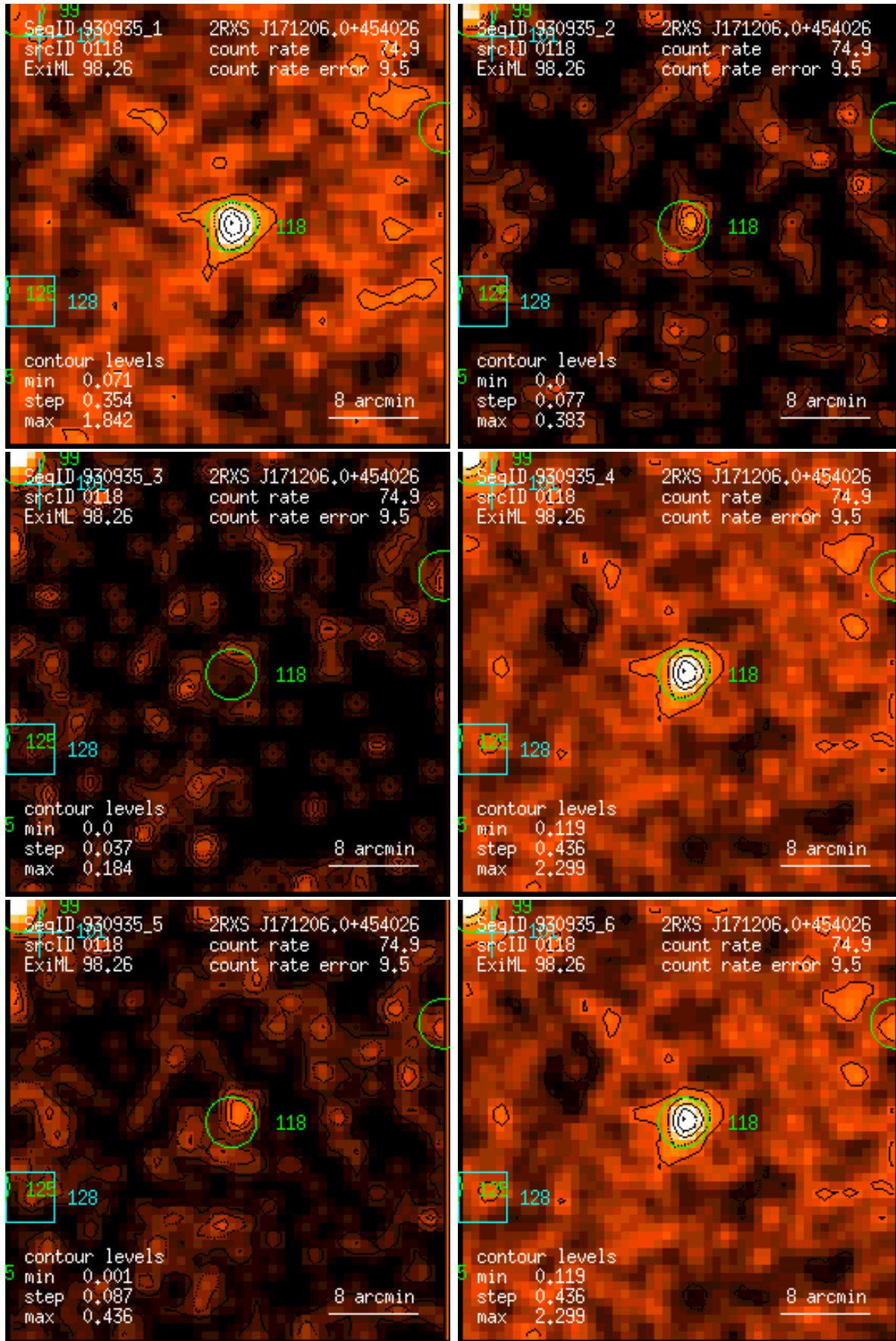
Figure 118: RASS 930935: detection 0118: band rate images, Gaussian filter: (1) PSPC channels 11 – 41, (2) 52 – 90, (3) 91 – 201, (4) 11 – 235, (5) 52 – 201, (6) 11 – 201. Broad band rates in counts/ks. Band rate contour levels in counts/ks/arcmin 2 .
