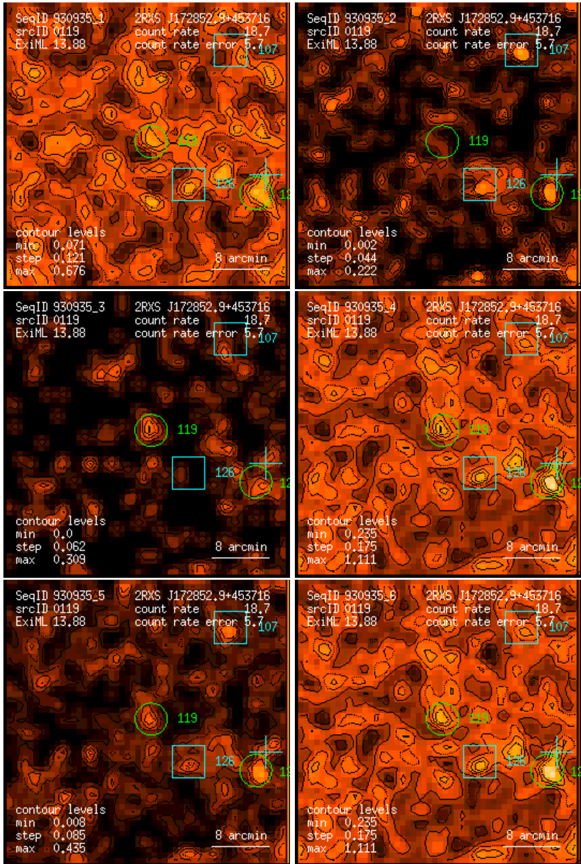
Figure 119: RASS 930935: detection 0119: band rate images, Gaussian filter: (1) PSPC channels 11 – 41, (2) 52 – 90, (3) 91 – 201, (4) 11 – 235, (5) 52 – 201, (6) 11 – 201. Broad band rates in counts/ks. Band rate contour levels in counts/ks/arcmin 2 .
