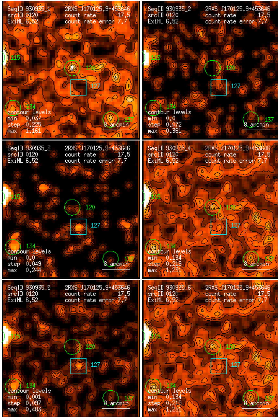
Figure 120: RASS 930935: detection 0120: band rate images, Gaussian filter: (1) PSPC channels 11 – 41, (2) 52 – 90, (3) 91 – 201, (4) 11 – 235, (5) 52 – 201, (6) 11 – 201. Broad band rates in counts/ks. Band rate contour levels in counts/ks/arcmin 2 .
