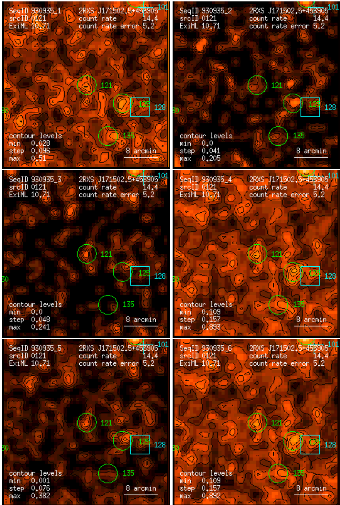
Figure 121: RASS 930935: detection 0121: band rate images, Gaussian filter: (1) PSPC channels 11 – 41, (2) 52 – 90, (3) 91 – 201, (4) 11 – 235, (5) 52 – 201, (6) 11 – 201. Broad band rates in counts/ks. Band rate contour levels in counts/ks/arcmin 2 .
