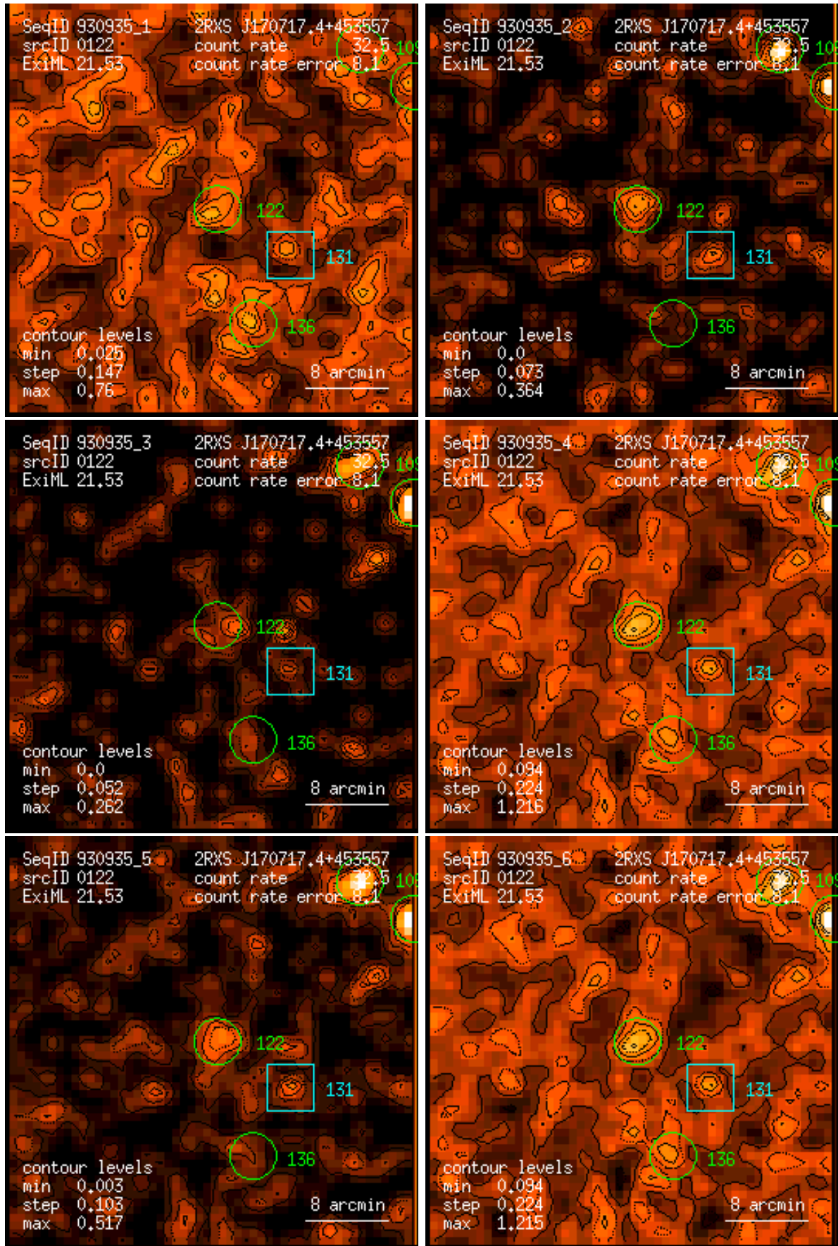
Figure 122: RASS 930935: detection 0122: band rate images, Gaussian filter: (1) PSPC channels 11 – 41, (2) 52 – 90, (3) 91 – 201, (4) 11 – 235, (5) 52 – 201, (6) 11 – 201. Broad band rates in counts/ks. Band rate contour levels in counts/ks/arcmin 2 .
