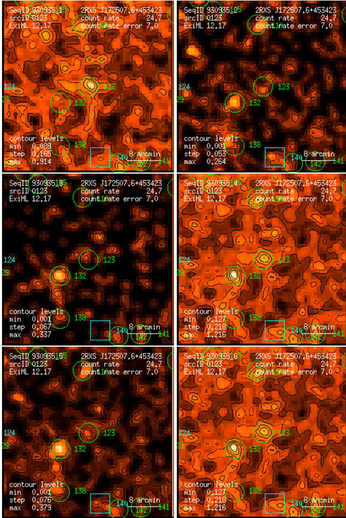
Figure 123: RASS 930935: detection 0123: band rate images, Gaussian filter: (1) PSPC channels 11 – 41, (2) 52 – 90, (3) 91 – 201, (4) 11 – 235, (5) 52 – 201, (6) 11 – 201. Broad band rates in counts/ks. Band rate contour levels in counts/ks/arcmin 2 .
