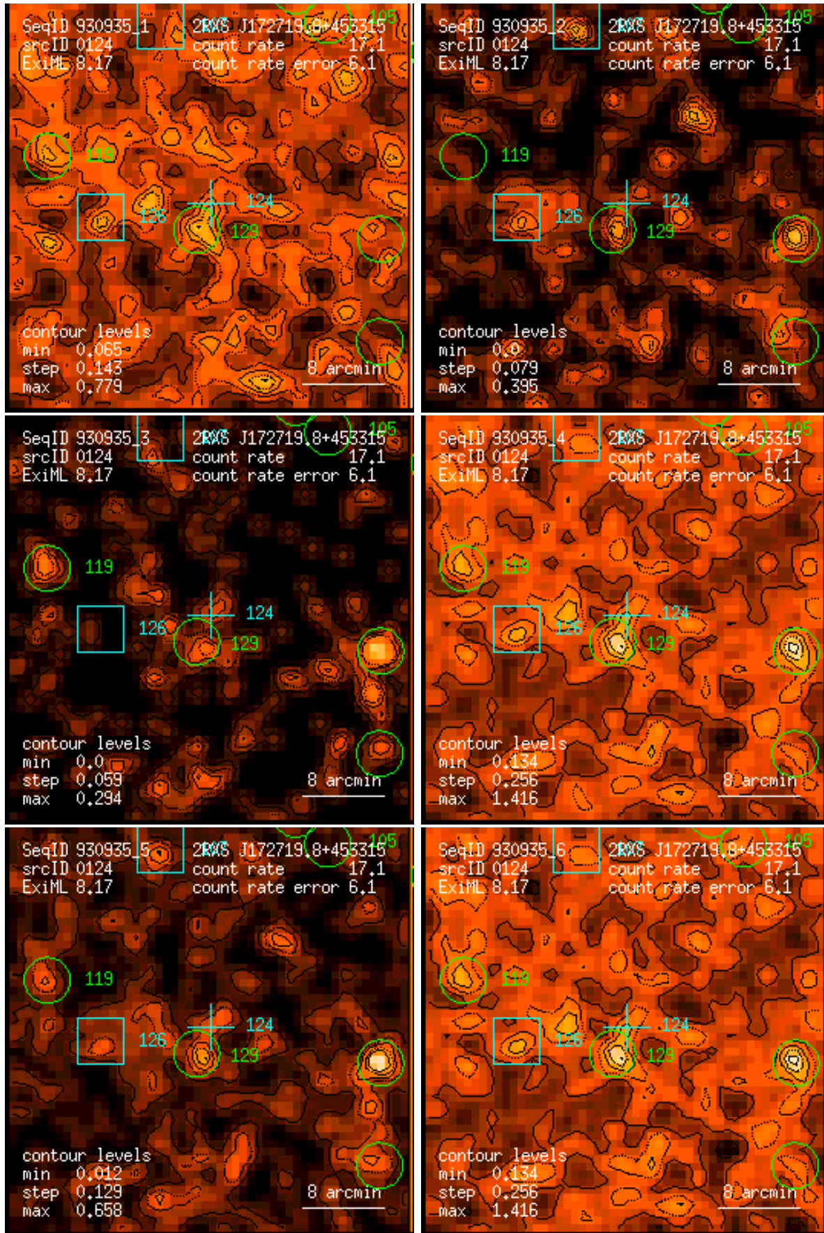
Figure 124: RASS 930935: detection 0124: band rate images, Gaussian filter: (1) PSPC channels 11 – 41, (2) 52 – 90, (3) 91 – 201, (4) 11 – 235, (5) 52 – 201, (6) 11 – 201. Broad band rates in counts/ks. Band rate contour levels in counts/ks/arcmin 2 .
