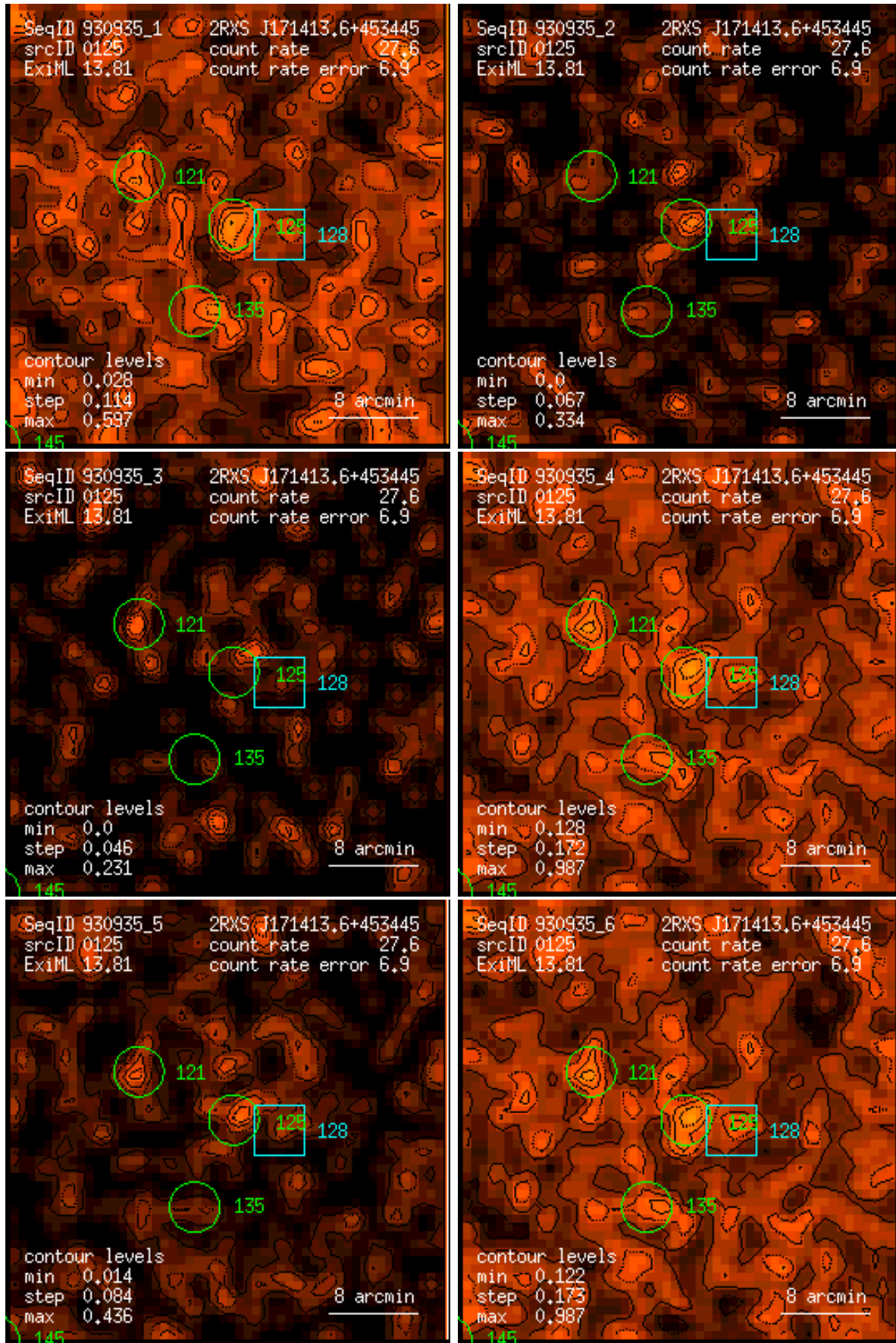
Figure 125: RASS 930935: detection 0125: band rate images, Gaussian filter: (1) PSPC channels 11 – 41, (2) 52 – 90, (3) 91 – 201, (4) 11 – 235, (5) 52 – 201, (6) 11 – 201. Broad band rates in counts/ks. Band rate contour levels in counts/ks/arcmin 2 .
