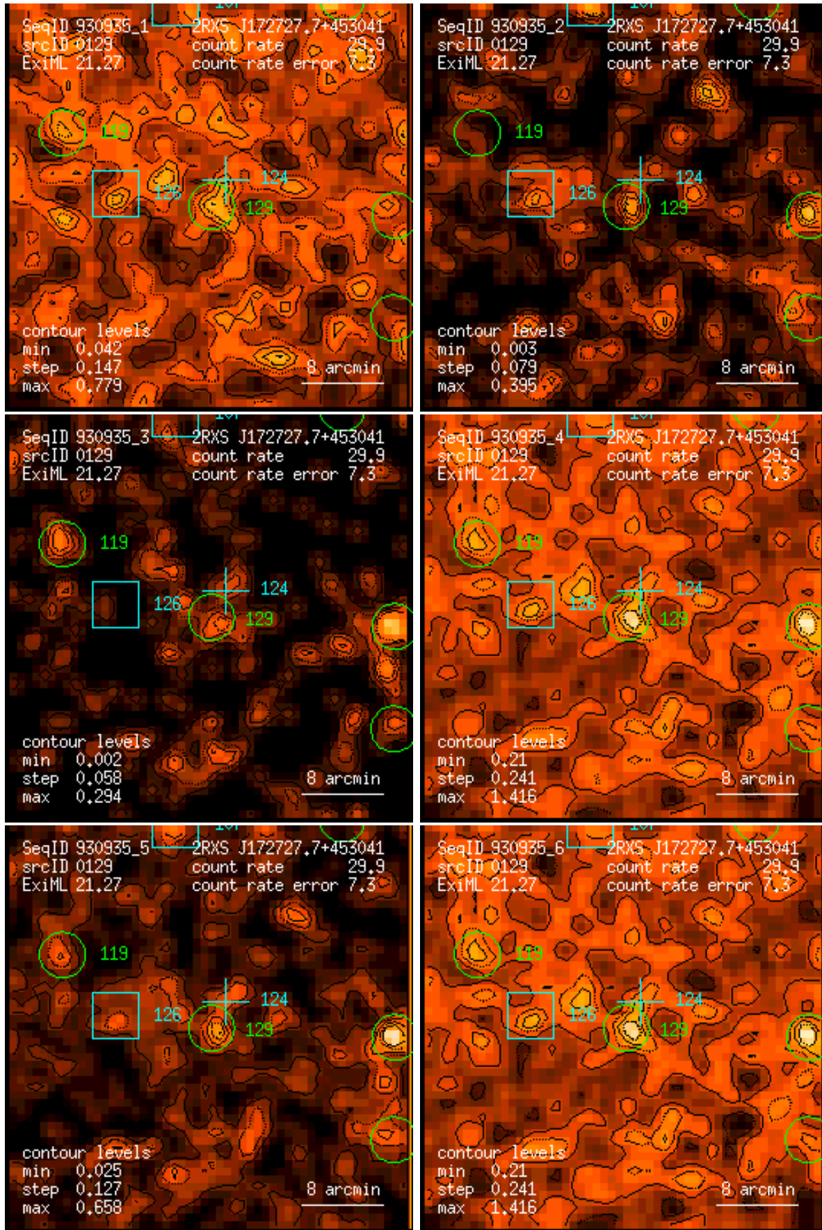
Figure 129: RASS 930935: detection 0129: band rate images, Gaussian filter: (1) PSPC channels 11 – 41, (2) 52 – 90, (3) 91 – 201, (4) 11 – 235, (5) 52 – 201, (6) 11 – 201. Broad band rates in counts/ks. Band rate contour levels in counts/ks/arcmin 2 .
